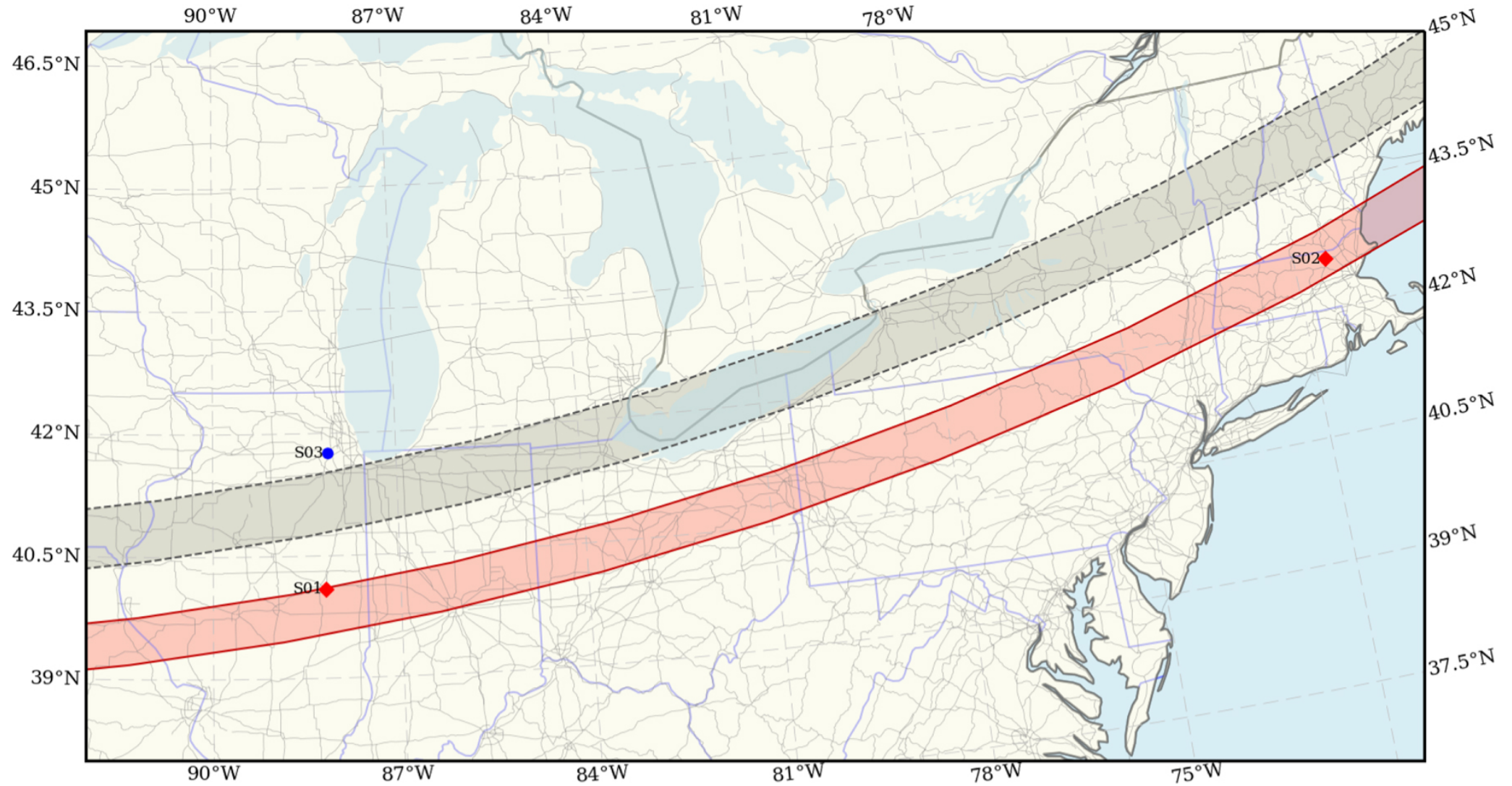
Figure 1. from Size and Shape of (11351) Leucus from Five Occultations null 2021 PSJ 2 202 doi:10.3847/PSJ/ac1f9b https://dx.doi.org/10.3847/PSJ/ac1f9b © 2021. The Author(s). Published by the American Astronomical Society.
