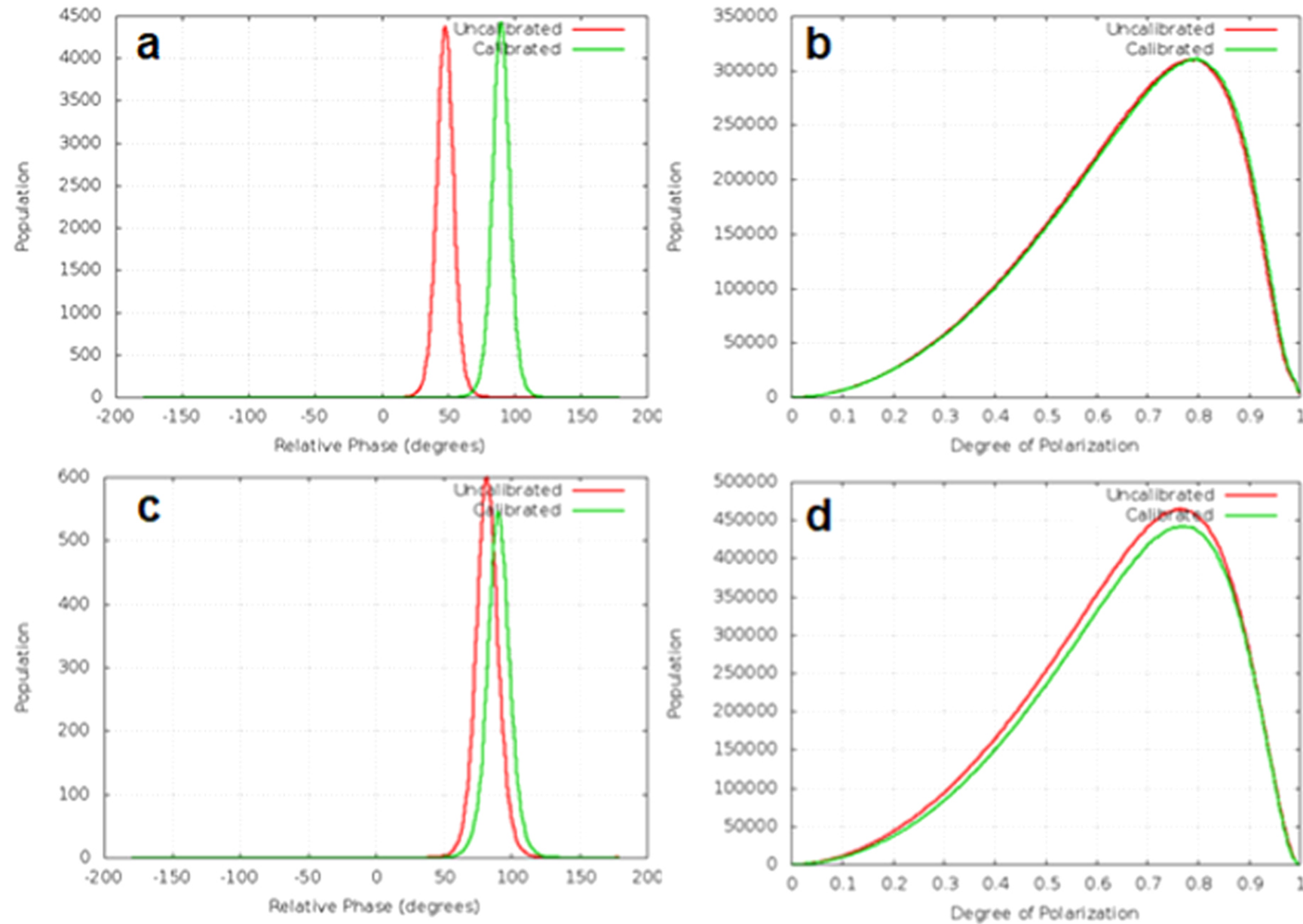
Figure 6. from Chandrayaan-2 Dual-frequency Synthetic Aperture Radar (DFSAR): Performance Characterization and Initial Results null 2021 PSJ 2 134 doi:10.3847/PSJ/abfdbf https://dx.doi.org/10.3847/PSJ/abfdbf © 2021. The Author(s). Published by the American Astronomical Society.
