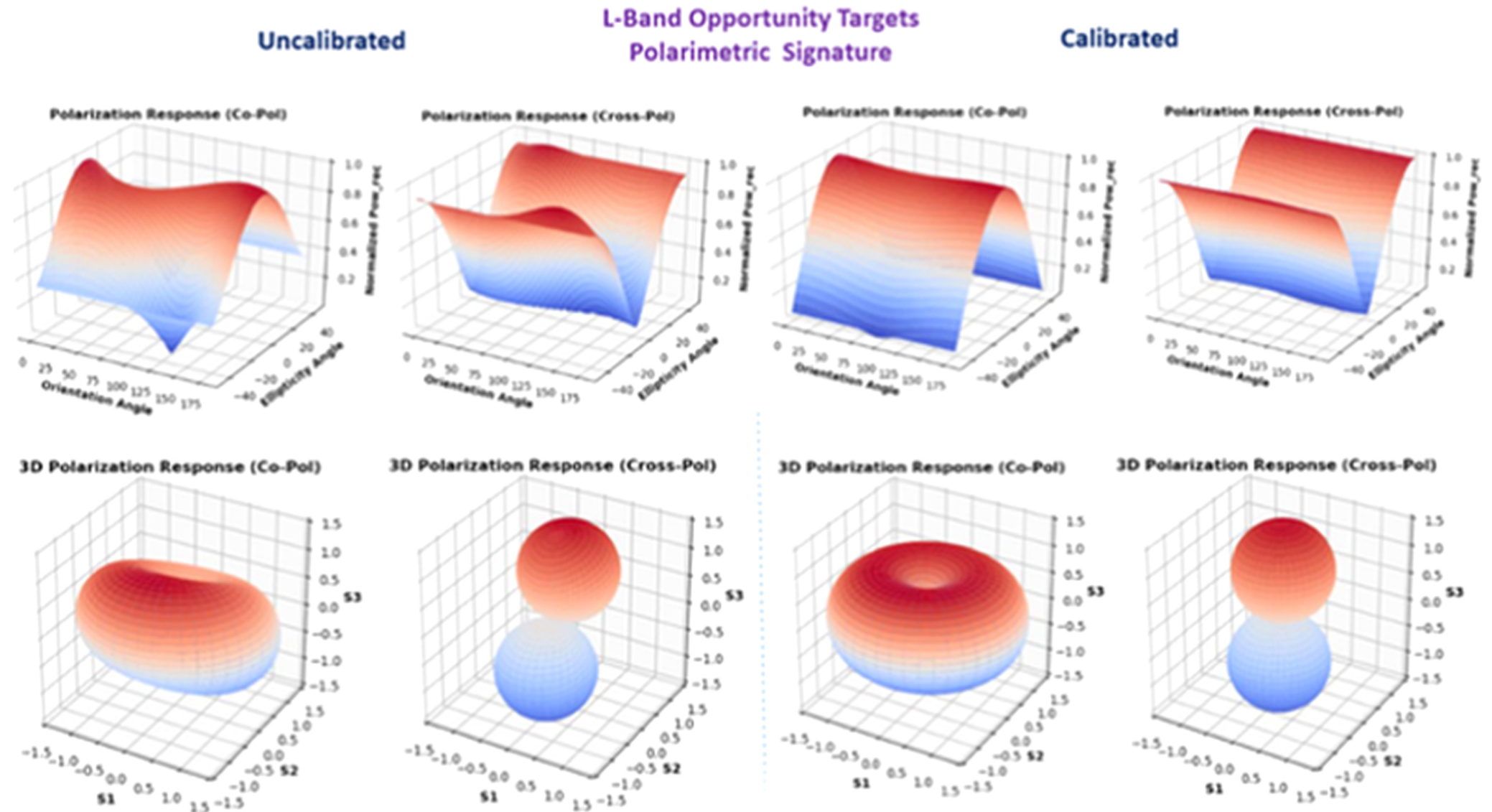
Figure 5. from Chandrayaan-2 Dual-frequency Synthetic Aperture Radar (DFSAR): Performance Characterization and Initial Results null 2021 PSJ 2 134 doi:10.3847/PSJ/abfdbf https://dx.doi.org/10.3847/PSJ/abfdbf © 2021. The Author(s). Published by the American Astronomical Society.
