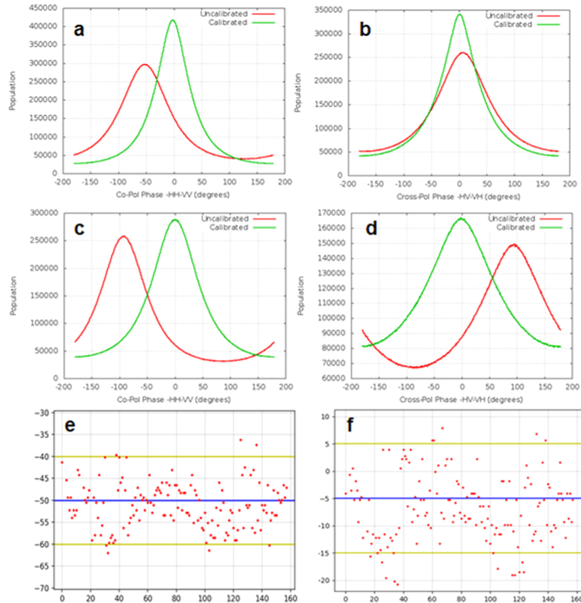
Figure 4. from Chandrayaan-2 Dual-frequency Synthetic Aperture Radar (DFSAR): Performance Characterization and Initial Results null 2021 PSJ 2 134 doi:10.3847/PSJ/abfdbf https://dx.doi.org/10.3847/PSJ/abfdbf © 2021. The Author(s). Published by the American Astronomical Society.
