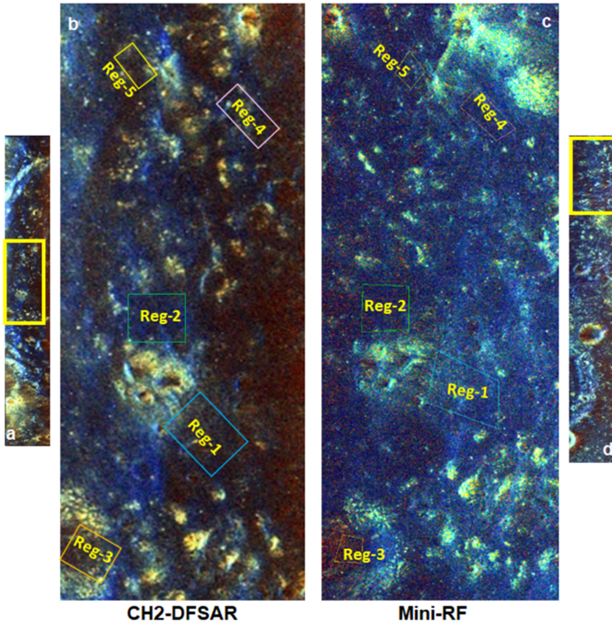
Figure 3. from Chandrayaan-2 Dual-frequency Synthetic Aperture Radar (DFSAR): Performance Characterization and Initial Results null 2021 PSJ 2 134 doi:10.3847/PSJ/abfdbf https://dx.doi.org/10.3847/PSJ/abfdbf © 2021. The Author(s). Published by the American Astronomical Society.
