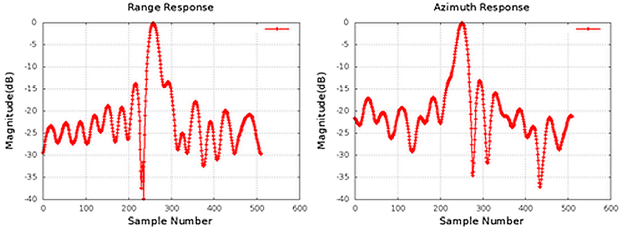
Figure 2. from Chandrayaan-2 Dual-frequency Synthetic Aperture Radar (DFSAR): Performance Characterization and Initial Results null 2021 PSJ 2 134 doi:10.3847/PSJ/abfdbf https://dx.doi.org/10.3847/PSJ/abfdbf © 2021. The Author(s). Published by the American Astronomical Society.
