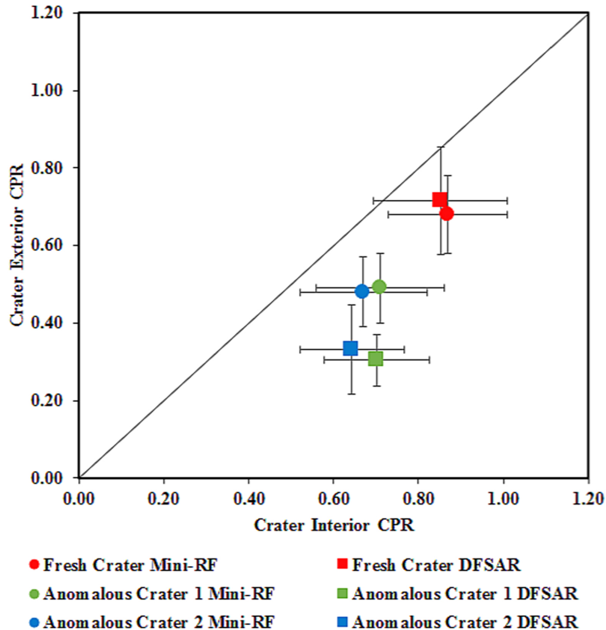
Figure 12. from Chandrayaan-2 Dual-frequency Synthetic Aperture Radar (DFSAR): Performance Characterization and Initial Results null 2021 PSJ 2 134 doi:10.3847/PSJ/abfdbf https://dx.doi.org/10.3847/PSJ/abfdbf © 2021. The Author(s). Published by the American Astronomical Society.
