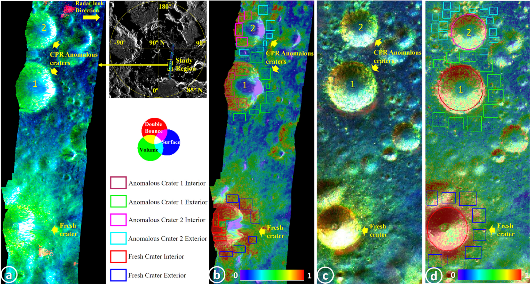
Figure 11. from Chandrayaan-2 Dual-frequency Synthetic Aperture Radar (DFSAR): Performance Characterization and Initial Results null 2021 PSJ 2 134 doi:10.3847/PSJ/abfdbf https://dx.doi.org/10.3847/PSJ/abfdbf © 2021. The Author(s). Published by the American Astronomical Society.
