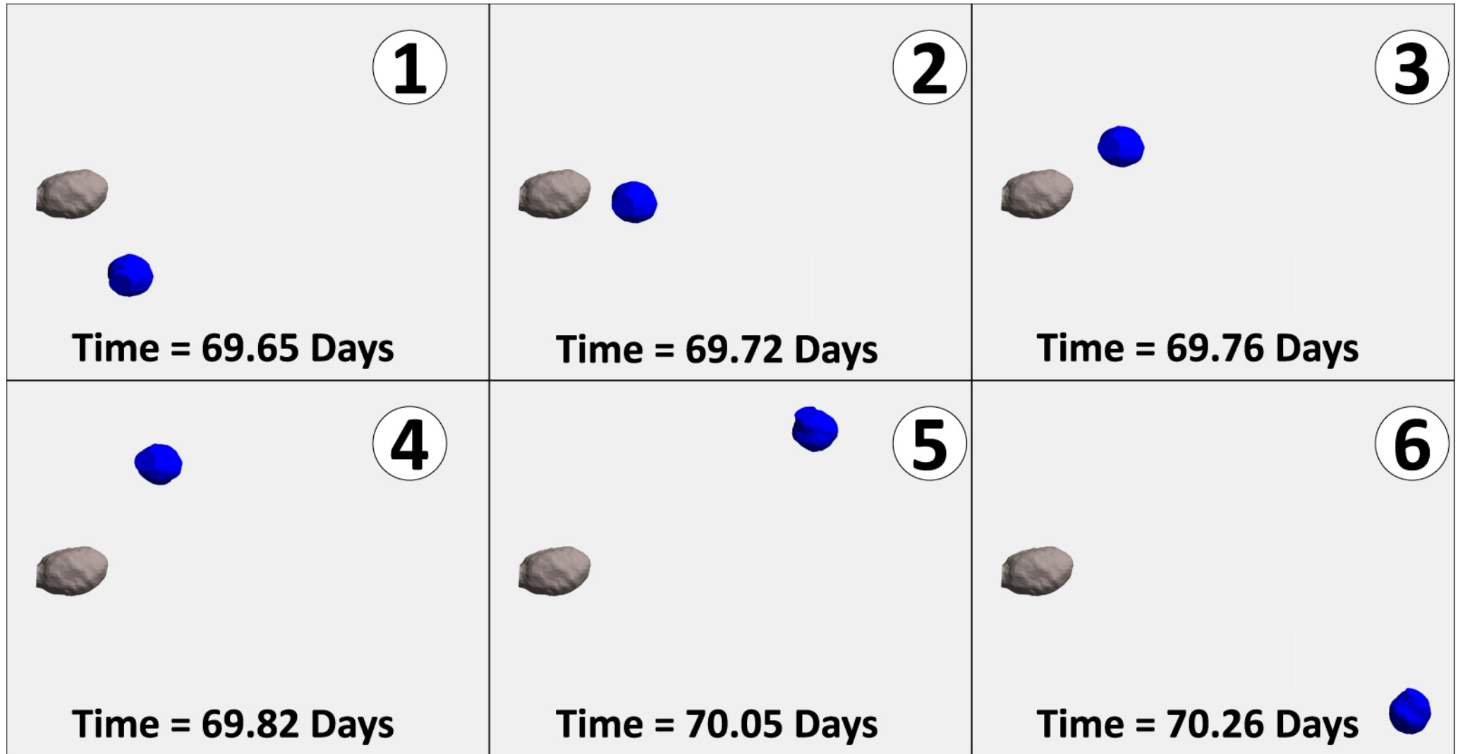
Figure 14. from High-fidelity Modeling of Rotationally Fissioned Asteroids null 2020 PSJ 1 25 doi:10.3847/PSJ/ab9a39 https://dx.doi.org/10.3847/PSJ/ab9a39 © 2020. The Author(s). Published by the American Astronomical Society.
