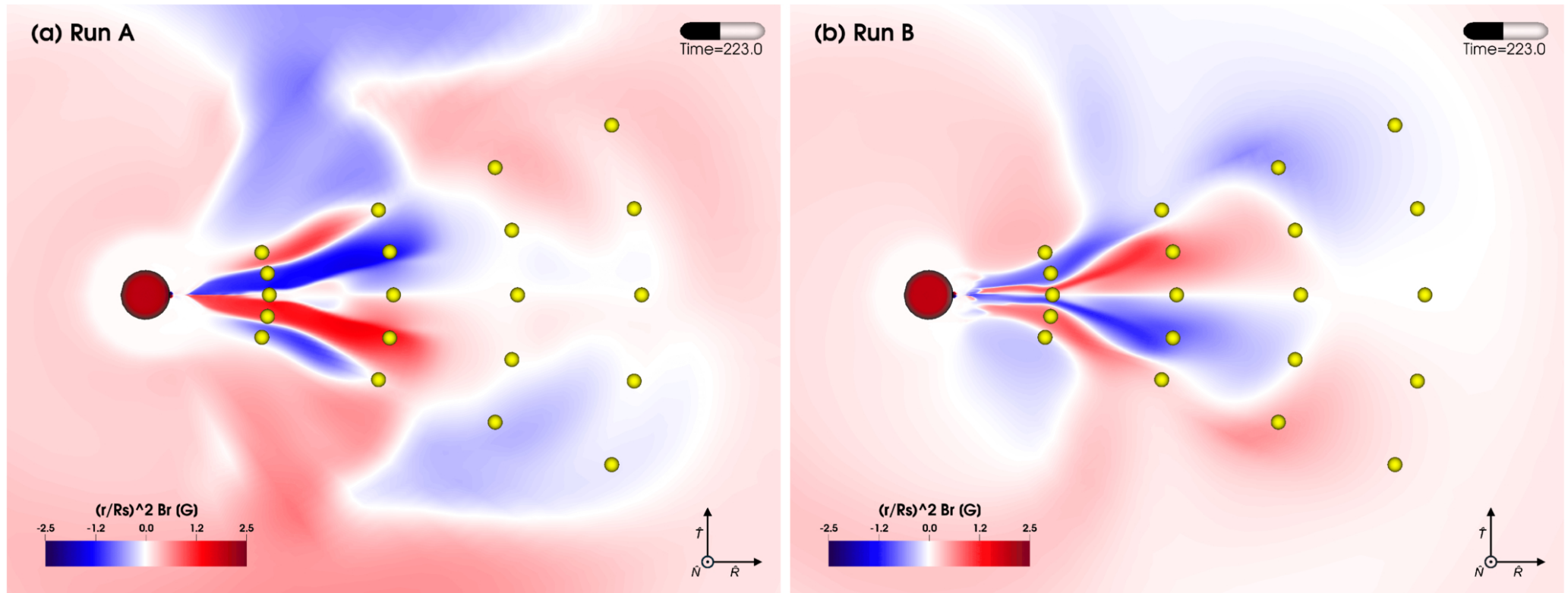
Figure 8. from Erika Palmerio et al 2026 Astrophys. J. Suppl. 286 doi:10.3847/1538-4365/aea6be https://dx.doi.org/10.3847/1538-4365/aea6be © 2026. The Author(s). Published by the American Astronomical Society.
