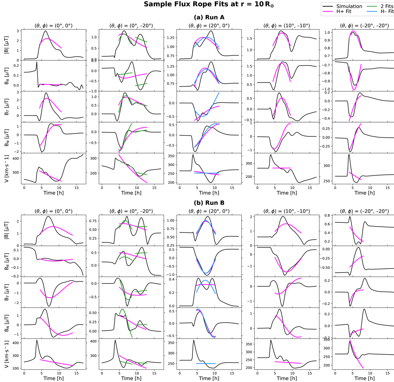
Figure 7. from Erika Palmerio et al 2026 Astrophys. J. Suppl. 286 doi:10.3847/1538-4365/aea6be https://dx.doi.org/10.3847/1538-4365/aea6be © 2026. The Author(s). Published by the American Astronomical Society.
