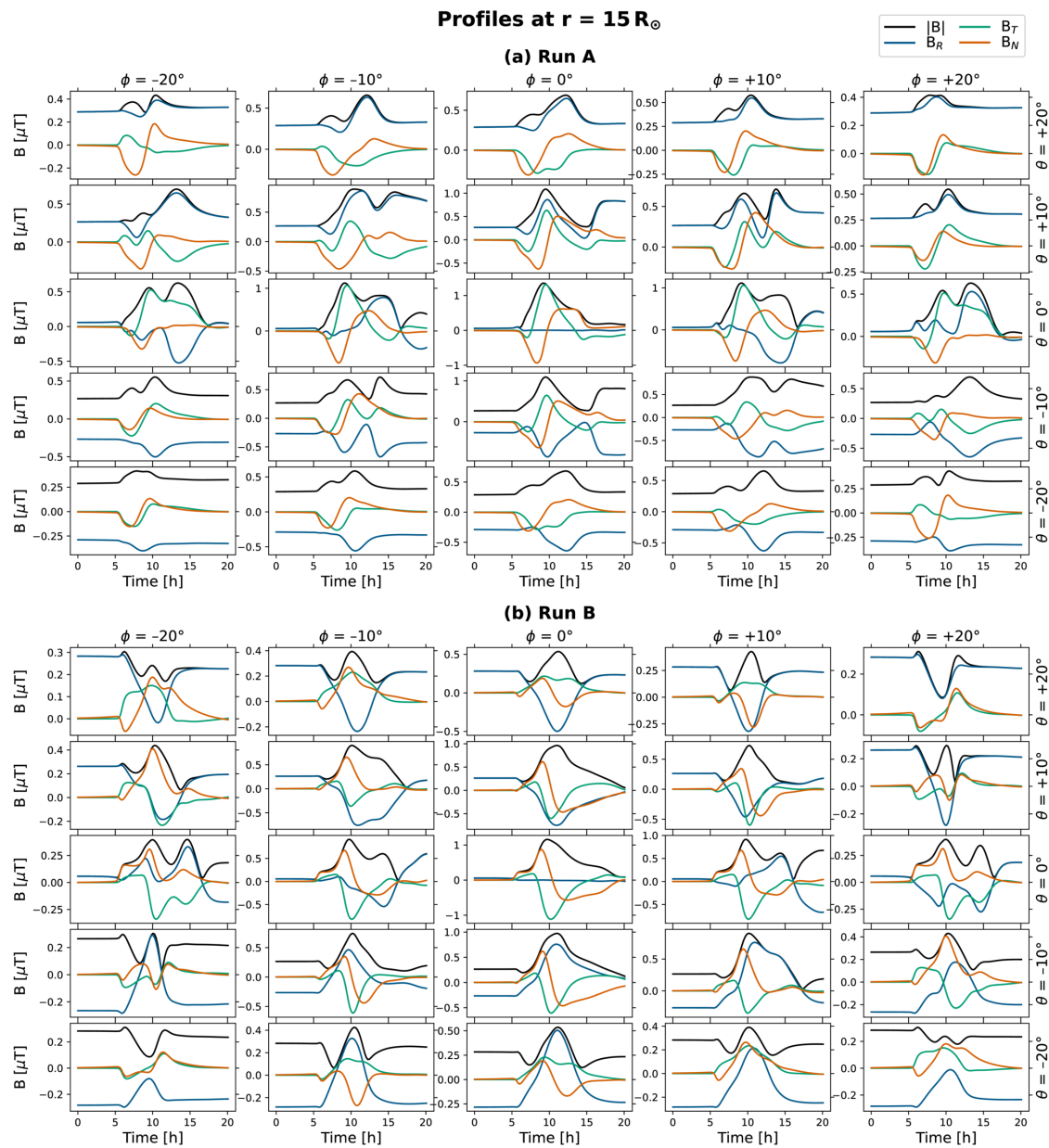
Figure 6. from Erika Palmerio et al 2026 Astrophys. J. Suppl. 286 doi:10.3847/1538-4365/aea6be https://dx.doi.org/10.3847/1538-4365/aea6be © 2026. The Author(s). Published by the American Astronomical Society.
