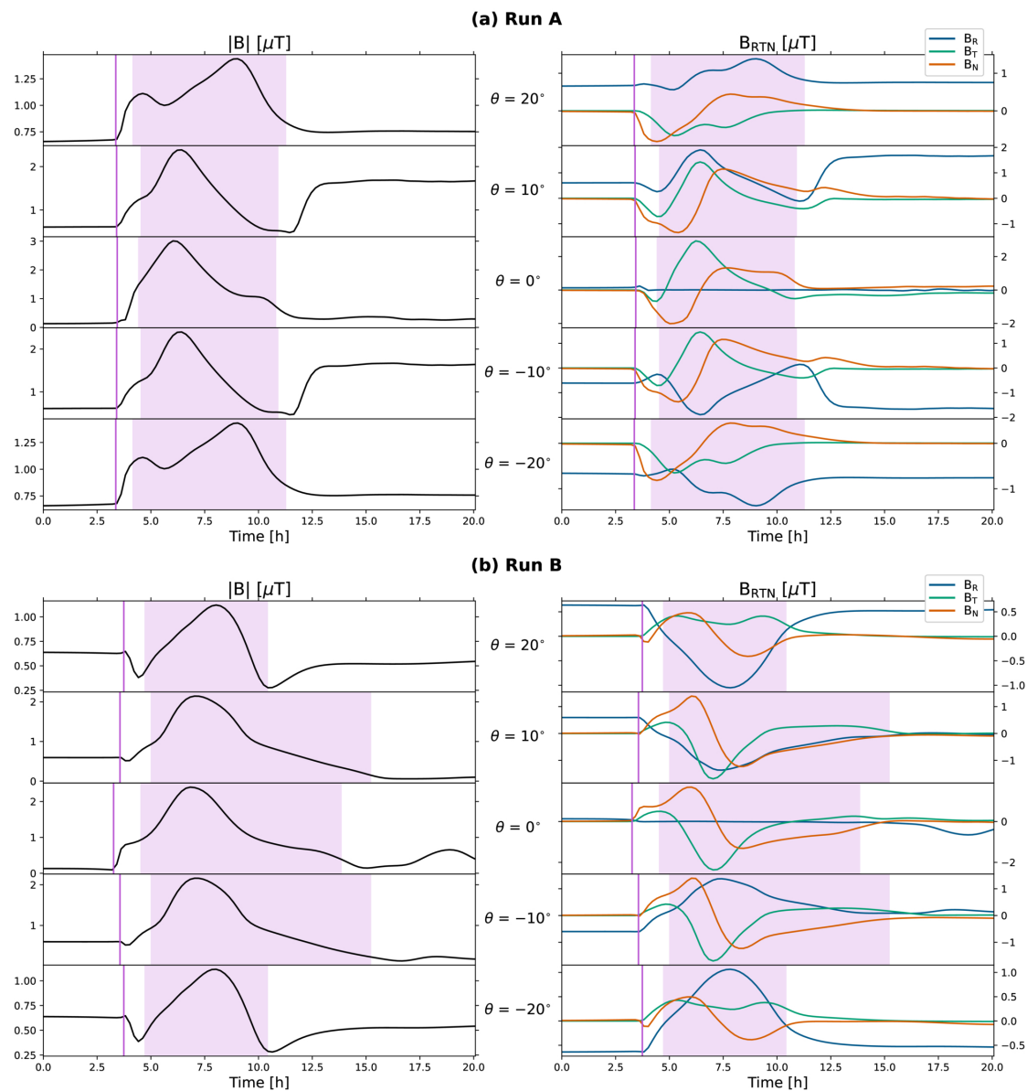
Figure 5. from Erika Palmerio et al 2026 Astrophys. J. Suppl. 286 doi:10.3847/1538-4365/aea6be https://dx.doi.org/10.3847/1538-4365/aea6be © 2026. The Author(s). Published by the American Astronomical Society.
