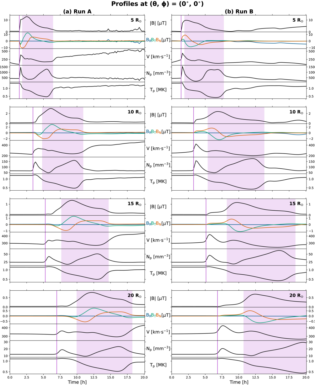
Figure 3. from Erika Palmerio et al 2026 Astrophys. J. Suppl. 286 doi:10.3847/1538-4365/aea6be https://dx.doi.org/10.3847/1538-4365/aea6be © 2026. The Author(s). Published by the American Astronomical Society.
