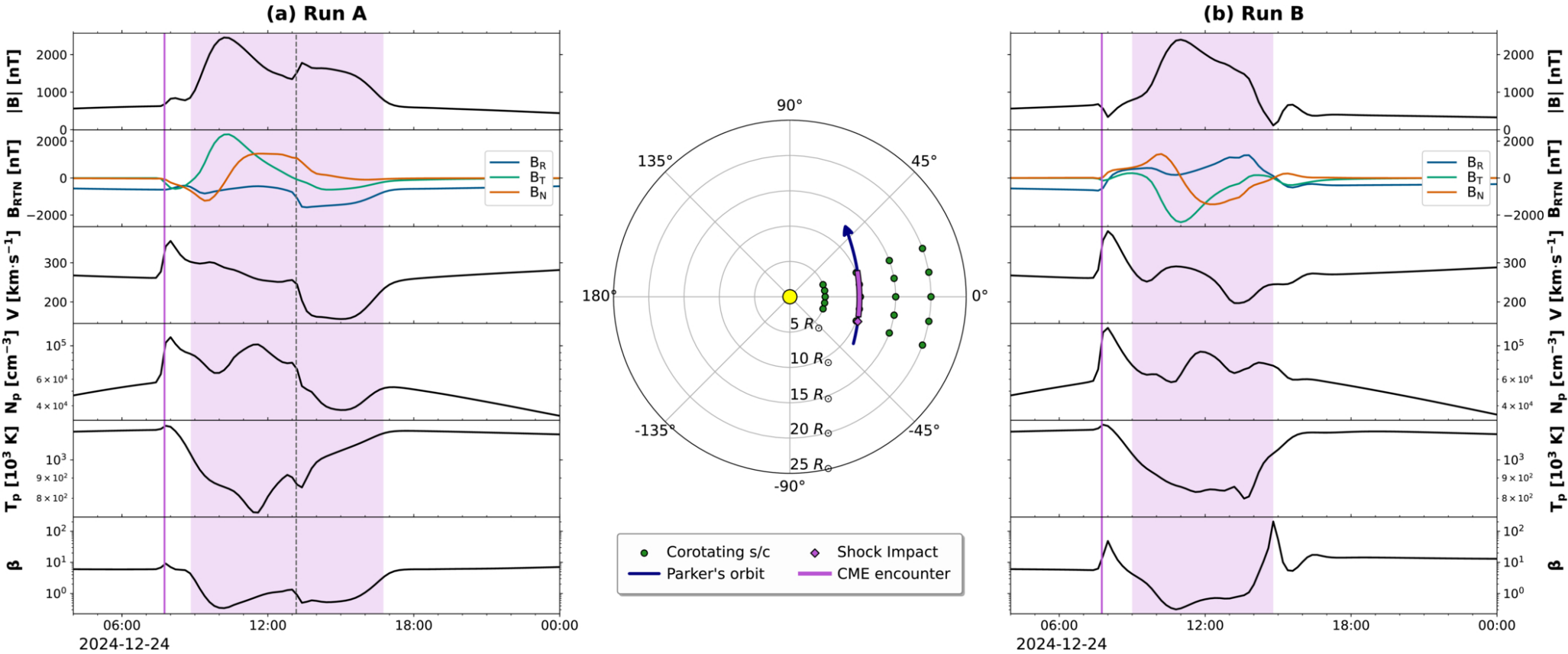
Figure 13. from Erika Palmerio et al 2026 Astrophys. J. Suppl. 286 doi:10.3847/1538-4365/aea6be https://dx.doi.org/10.3847/1538-4365/aea6be © 2026. The Author(s). Published by the American Astronomical Society.
