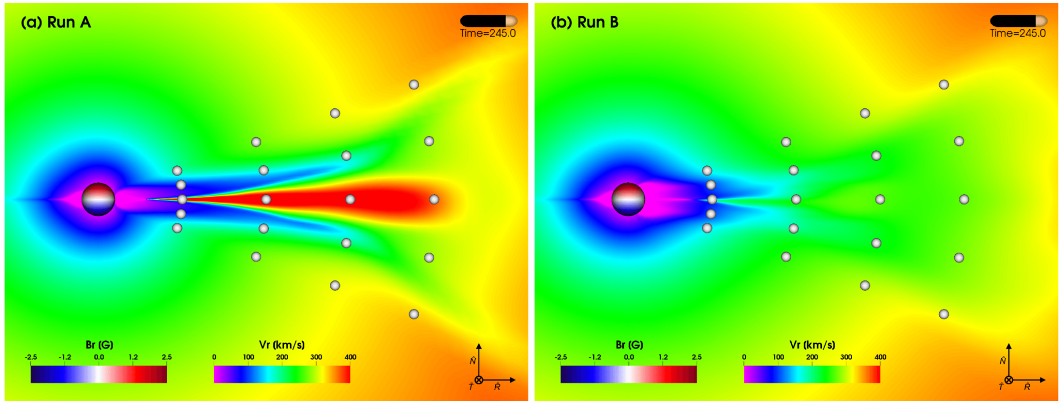
Figure 12. from Erika Palmerio et al 2026 Astrophys. J. Suppl. 286 doi:10.3847/1538-4365/aea6be https://dx.doi.org/10.3847/1538-4365/aea6be © 2026. The Author(s). Published by the American Astronomical Society.
