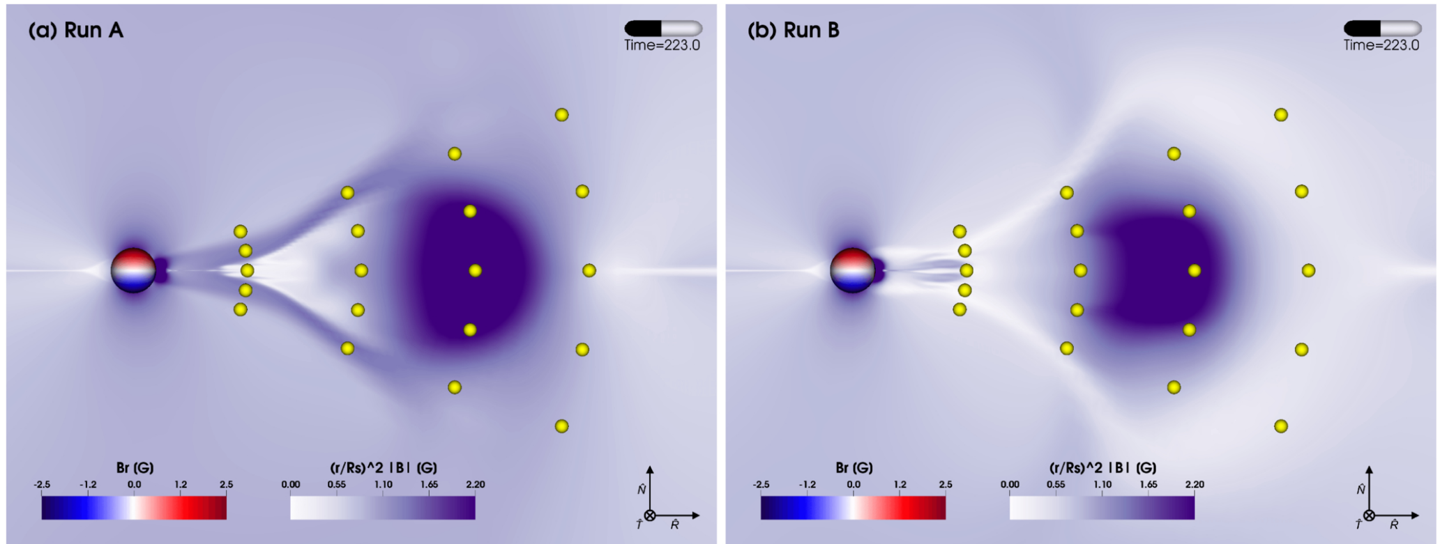
Figure 11. from Erika Palmerio et al 2026 Astrophys. J. Suppl. 286 doi:10.3847/1538-4365/aea6be https://dx.doi.org/10.3847/1538-4365/aea6be © 2026. The Author(s). Published by the American Astronomical Society.
