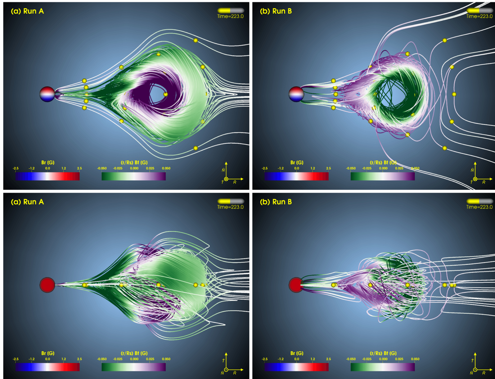
Figure 10. from Erika Palmerio et al 2026 Astrophys. J. Suppl. 286 doi:10.3847/1538-4365/aea6be https://dx.doi.org/10.3847/1538-4365/aea6be © 2026. The Author(s). Published by the American Astronomical Society.
