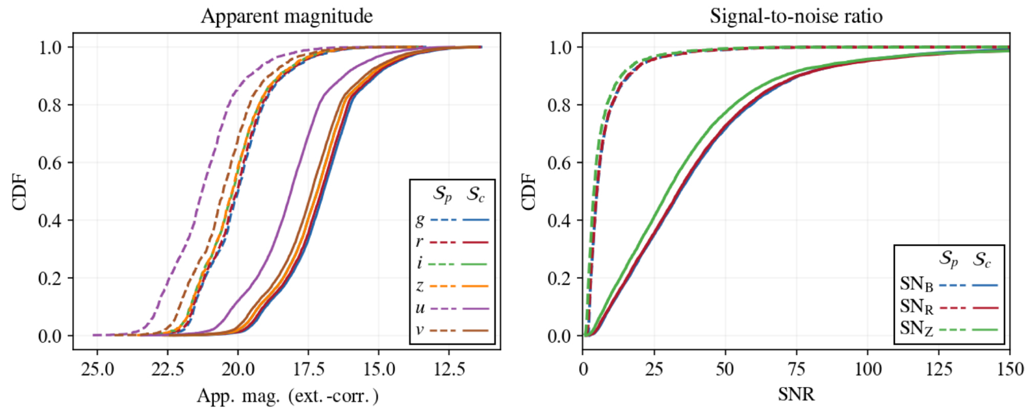
Figure 9. from Shuai Zhang et al 2026 Astrophys. J. Suppl. 286 doi:10.3847/1538-4365/aea410 https://dx.doi.org/10.3847/1538-4365/aea410 © 2026. The Author(s). Published by the American Astronomical Society.
