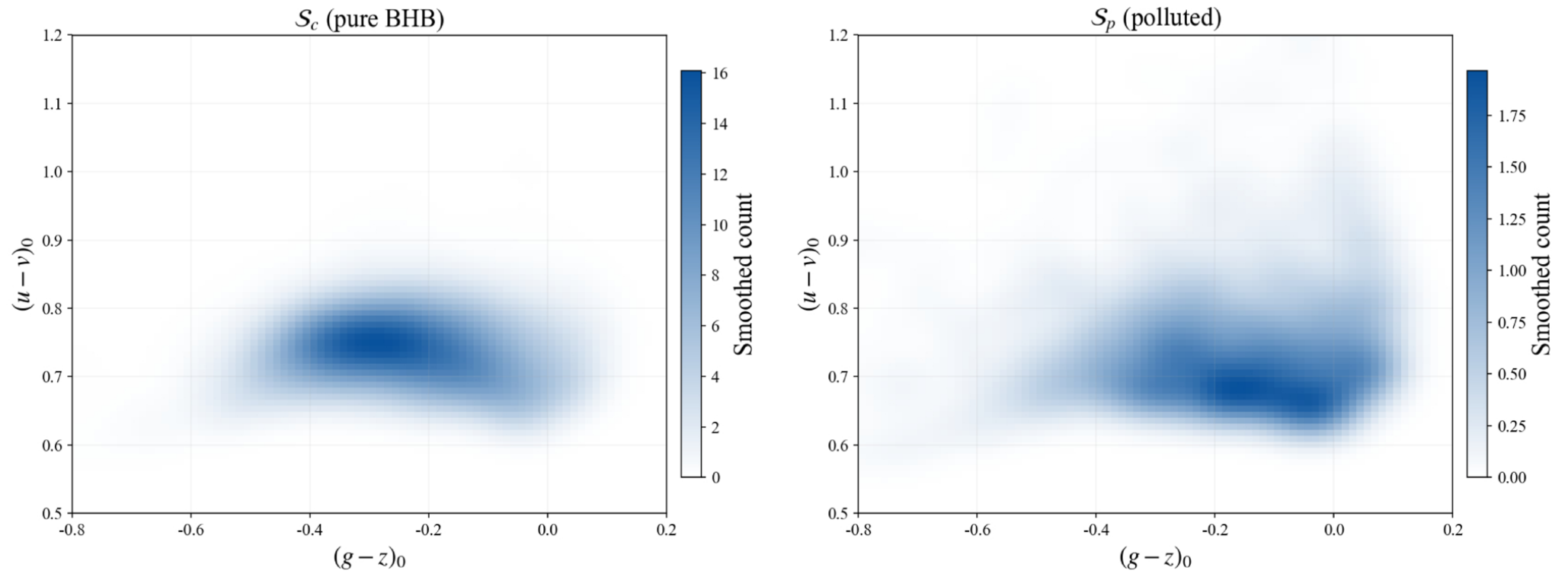
Figure 8. from Shuai Zhang et al 2026 Astrophys. J. Suppl. 286 doi:10.3847/1538-4365/aea410 https://dx.doi.org/10.3847/1538-4365/aea410 © 2026. The Author(s). Published by the American Astronomical Society.
