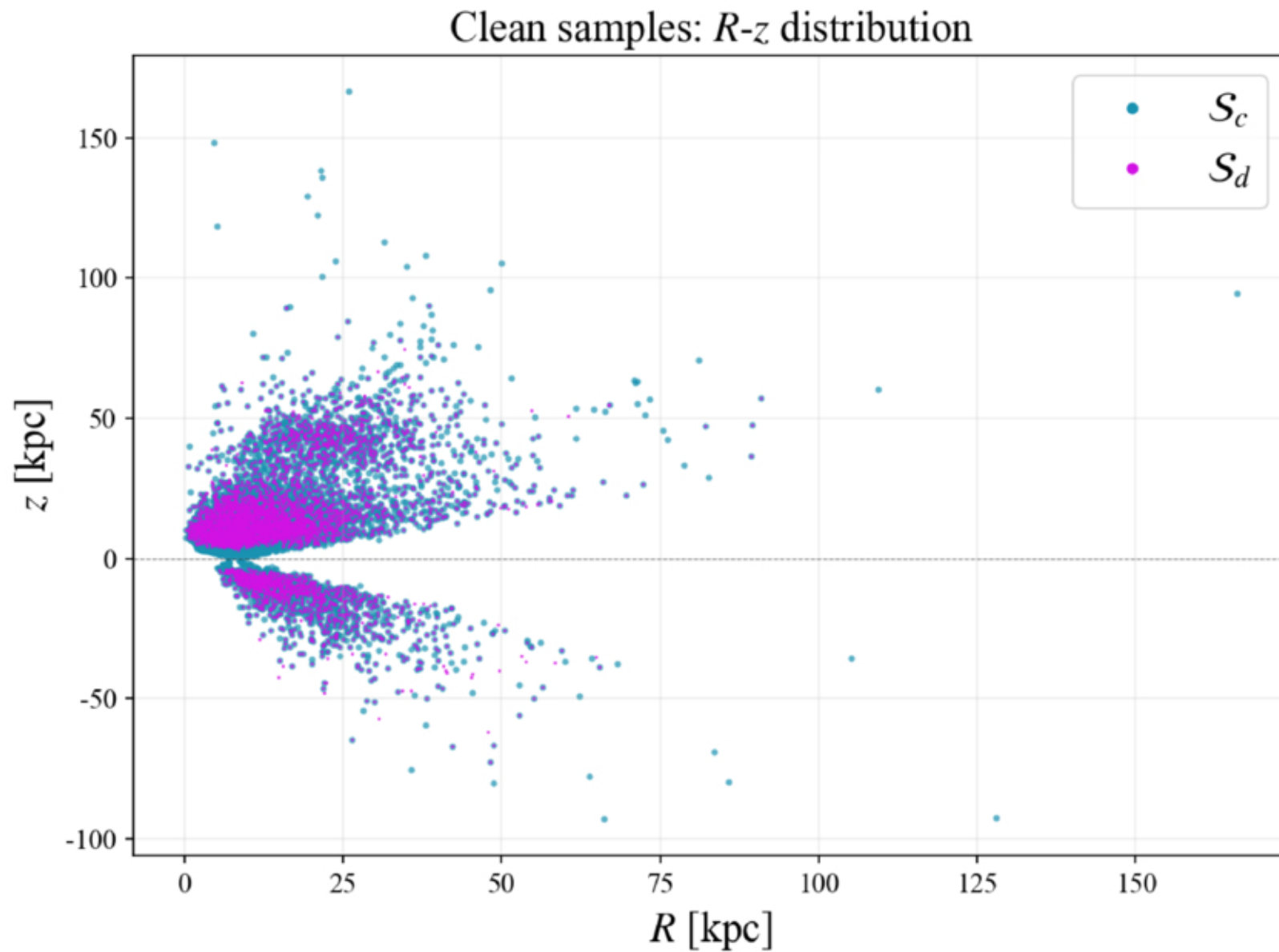
Figure 7. from Shuai Zhang et al 2026 Astrophys. J. Suppl. 286 doi:10.3847/1538-4365/aea410 https://dx.doi.org/10.3847/1538-4365/aea410 © 2026. The Author(s). Published by the American Astronomical Society.
