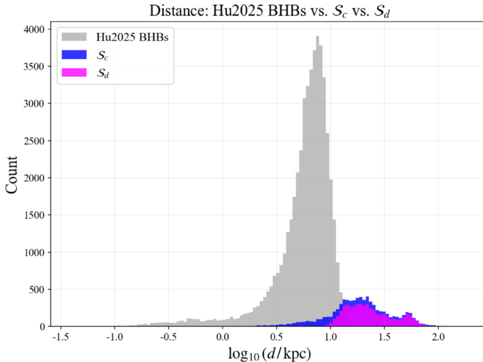
Figure 6. from Shuai Zhang et al 2026 Astrophys. J. Suppl. 286 doi:10.3847/1538-4365/aea410 https://dx.doi.org/10.3847/1538-4365/aea410 © 2026. The Author(s). Published by the American Astronomical Society.
