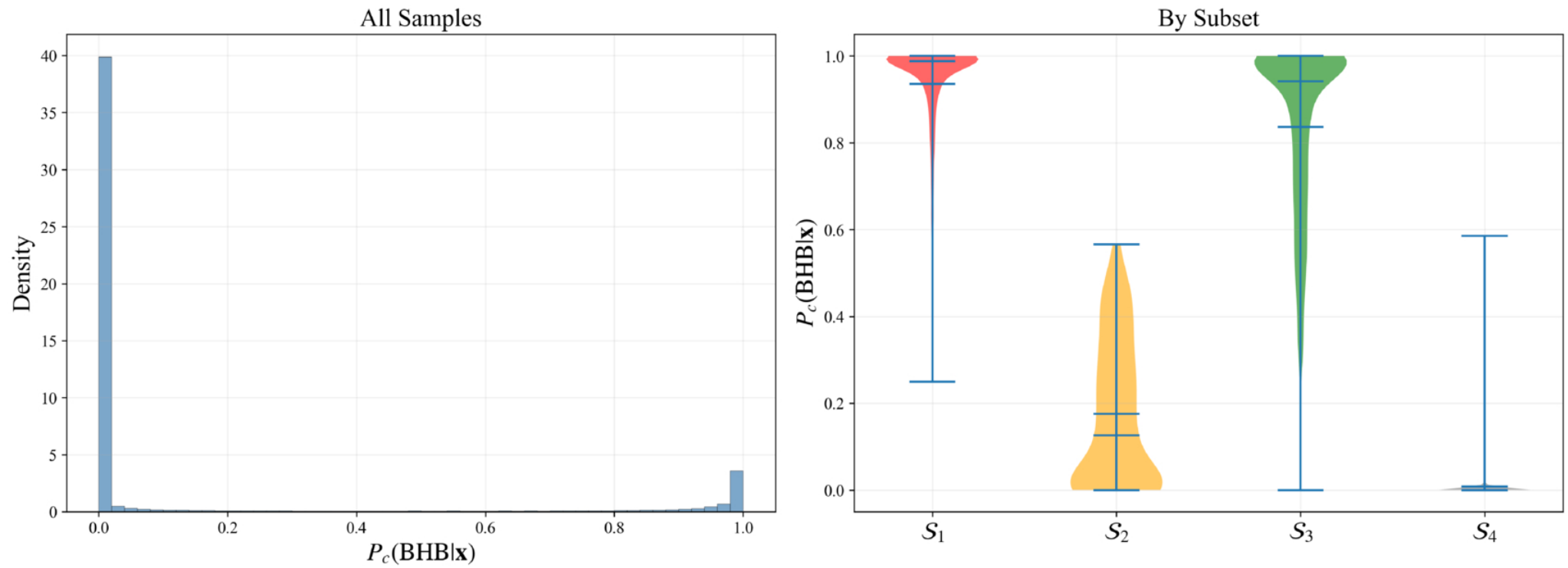
Figure 4. from Shuai Zhang et al 2026 Astrophys. J. Suppl. 286 doi:10.3847/1538-4365/aea410 https://dx.doi.org/10.3847/1538-4365/aea410 © 2026. The Author(s). Published by the American Astronomical Society.
