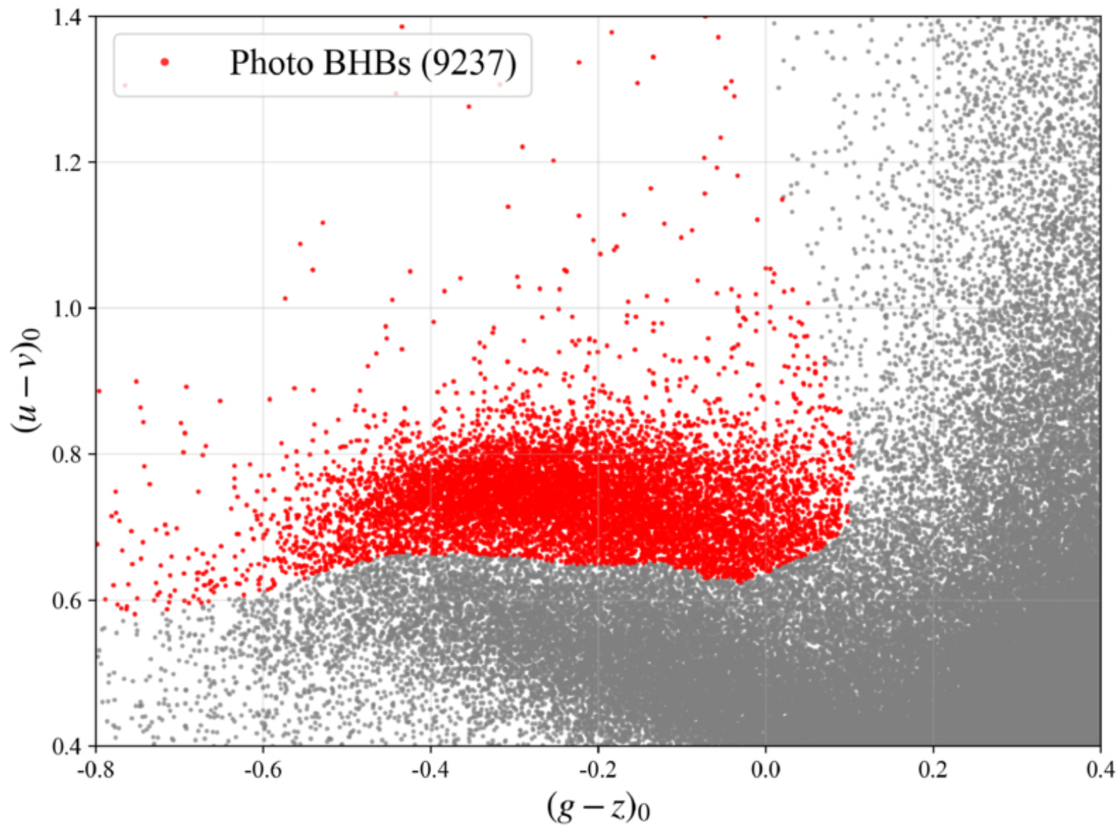
Figure 2. from Shuai Zhang et al 2026 Astrophys. J. Suppl. 286 doi:10.3847/1538-4365/aea410 https://dx.doi.org/10.3847/1538-4365/aea410 © 2026. The Author(s). Published by the American Astronomical Society.
