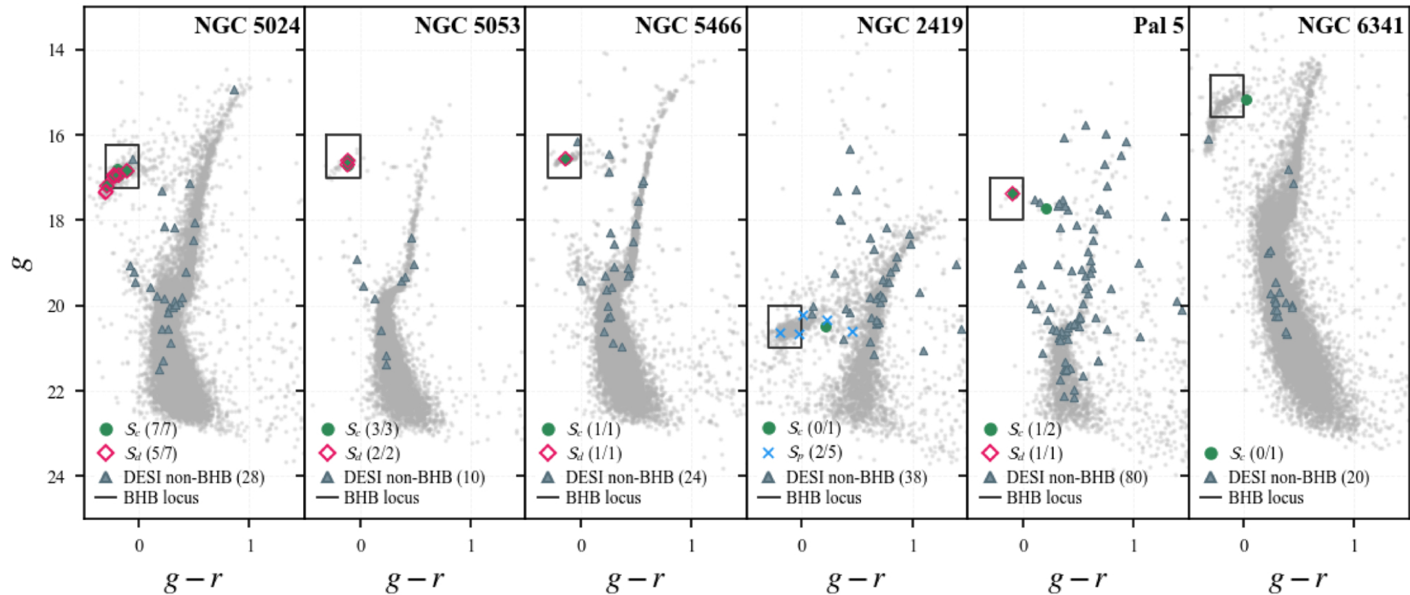
Figure 10. from Shuai Zhang et al 2026 Astrophys. J. Suppl. 286 doi:10.3847/1538-4365/aea410 https://dx.doi.org/10.3847/1538-4365/aea410 © 2026. The Author(s). Published by the American Astronomical Society.
