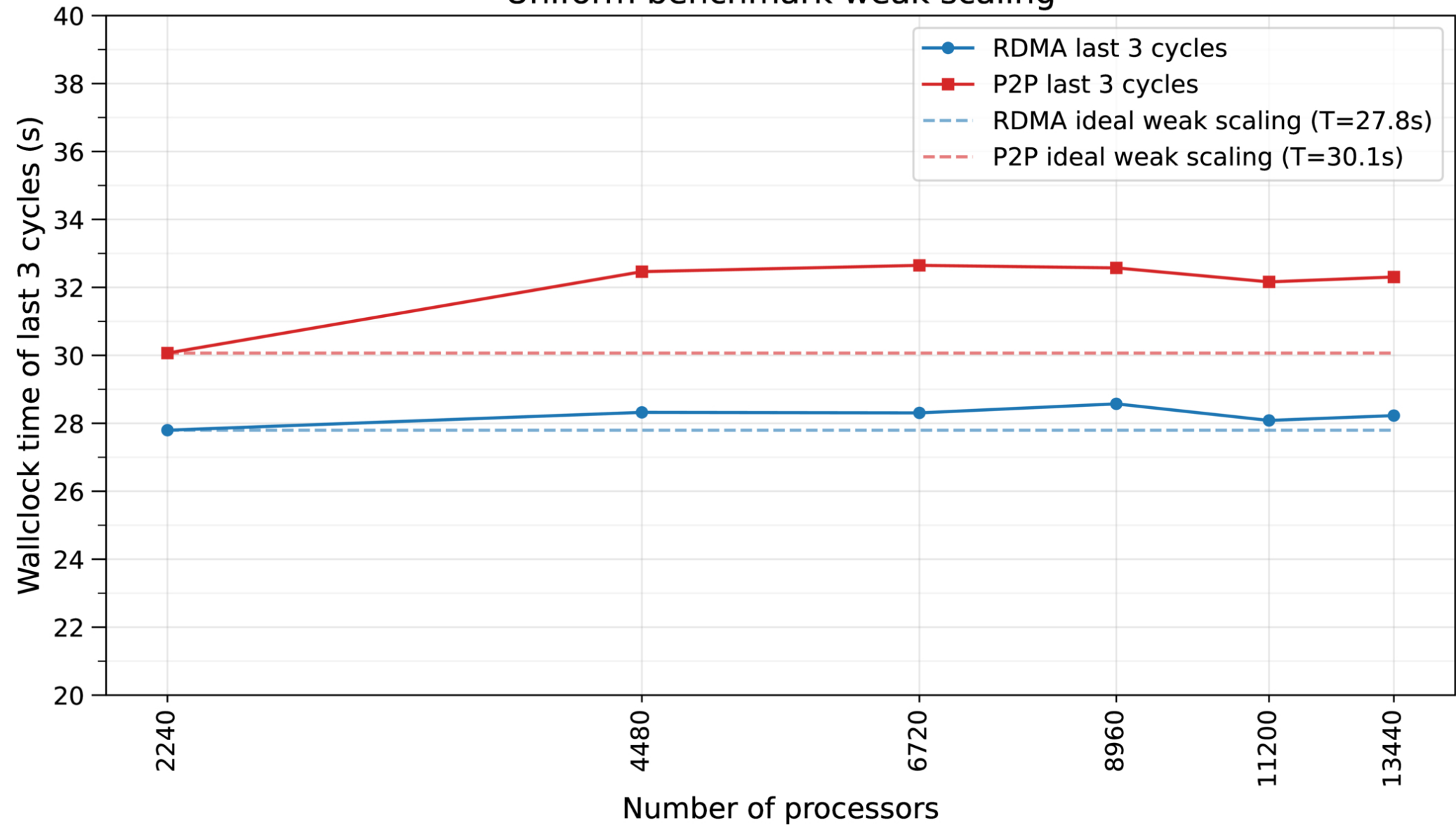
Figure 8. from Maor Mizrahi et al 2026 Astrophys. J. Suppl. 286 doi:10.3847/1538-4365/aea3f8 https://dx.doi.org/10.3847/1538-4365/aea3f8 © 2026. The Author(s). Published by the American Astronomical Society.
