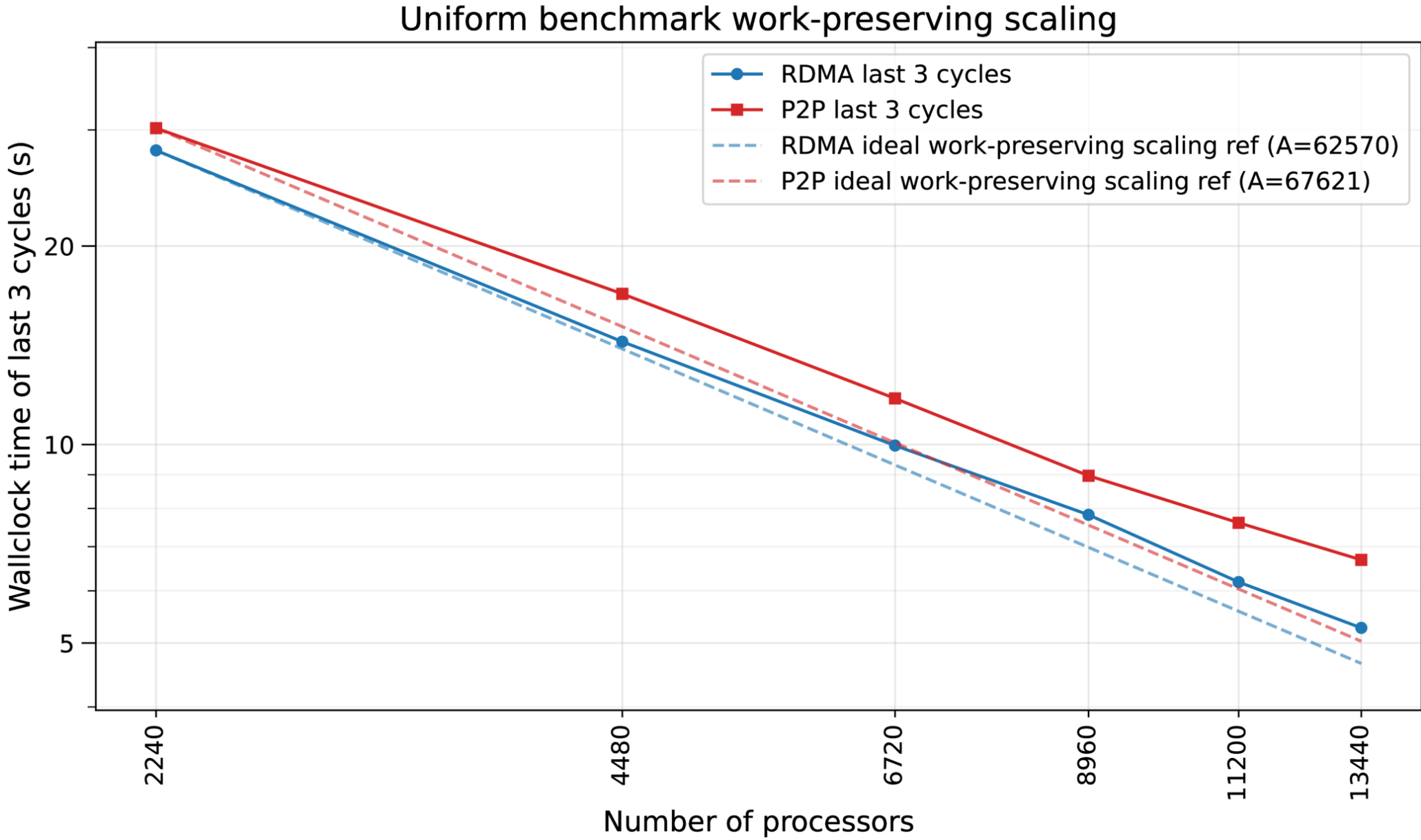
Figure 7. from Maor Mizrachi et al 2026 Astrophys. J. Suppl. 286 doi:10.3847/1538-4365/aea3f8 https://dx.doi.org/10.3847/1538-4365/aea3f8 © 2026. The Author(s). Published by the American Astronomical Society.
