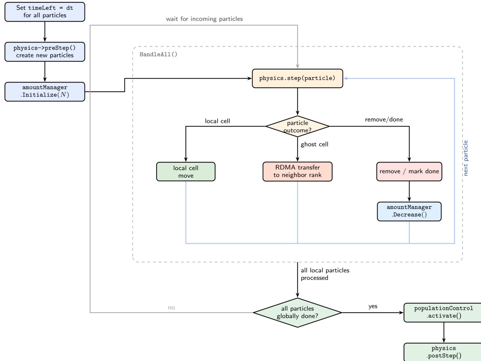
Figure 2. from Maor Mizrahi et al 2026 Astrophys. J. Suppl. 286 doi:10.3847/1538-4365/aea3f8 https://dx.doi.org/10.3847/1538-4365/aea3f8 © 2026. The Author(s). Published by the American Astronomical Society.
