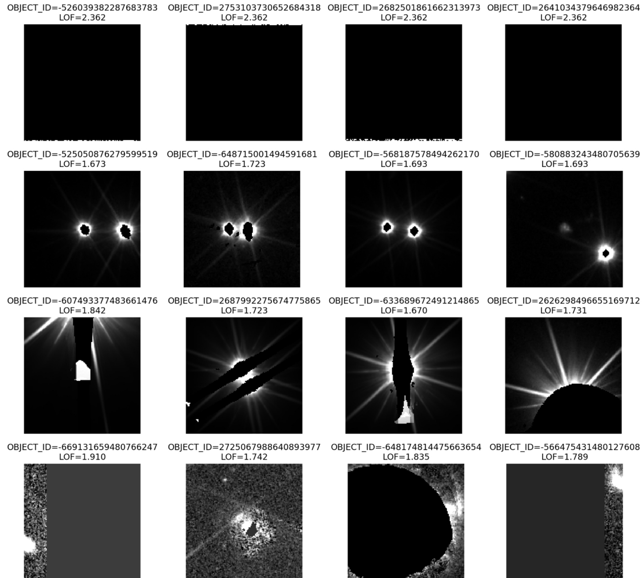
Figure 7. from Jinhui Xie et al 2026 Astrophys. J. Suppl. 287 doi:10.3847/1538-4365/aea223 https://dx.doi.org/10.3847/1538-4365/aea223 © 2026. The Author(s). Published by the American Astronomical Society.
