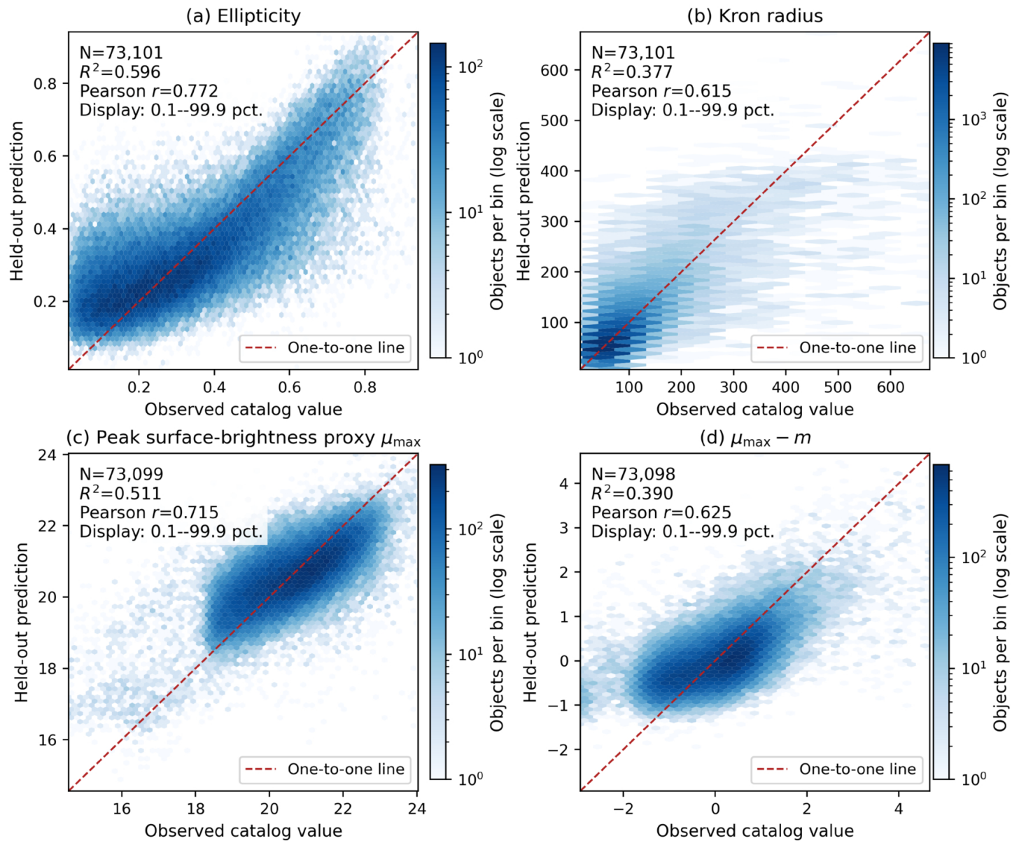
Figure 3. from Jinhui Xie et al 2026 Astrophys. J. Suppl. 287 doi:10.3847/1538-4365/aea223 https://dx.doi.org/10.3847/1538-4365/aea223 © 2026. The Author(s). Published by the American Astronomical Society.
