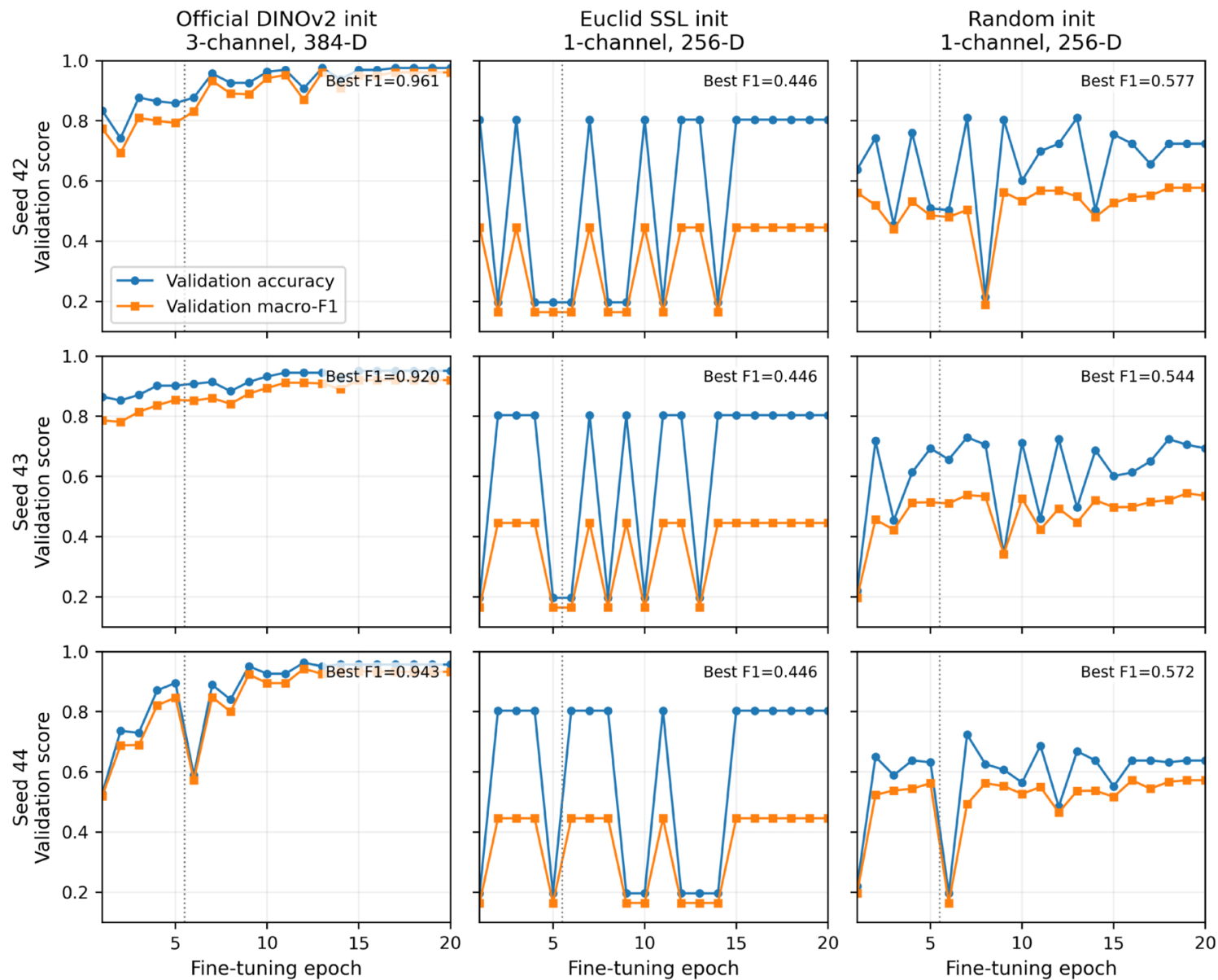
Figure A1. from Jinhui Xie et al 2026 Astrophys. J. Suppl. 287 doi:10.3847/1538-4365/aea223 https://dx.doi.org/10.3847/1538-4365/aea223 © 2026. The Author(s). Published by the American Astronomical Society.
