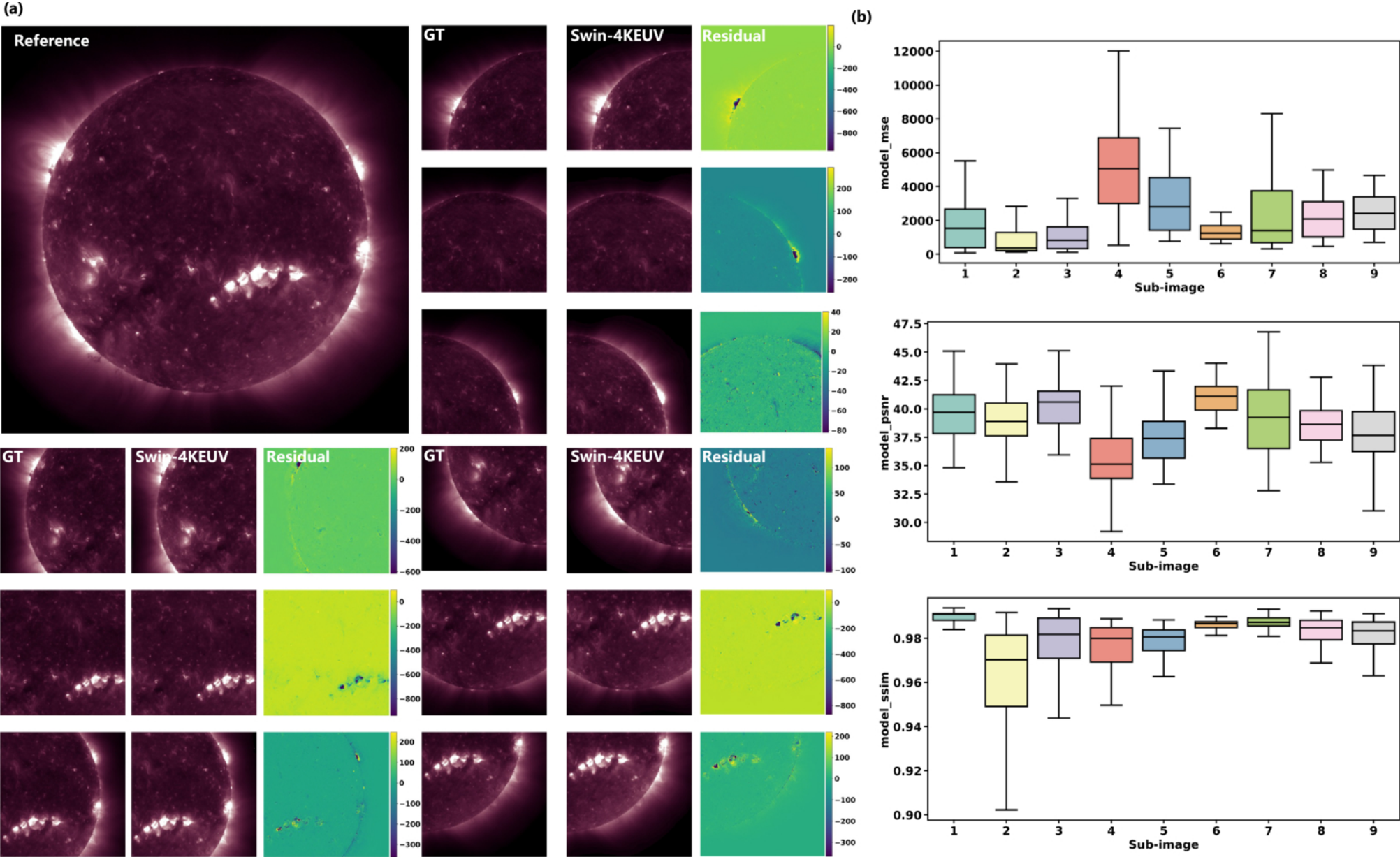
Figure 5. from Hao Li et al 2026 Astrophys. J. Suppl. 287 doi:10.3847/1538-4365/aea219 https://dx.doi.org/10.3847/1538-4365/aea219 © 2026. The Author(s). Published by the American Astronomical Society.
