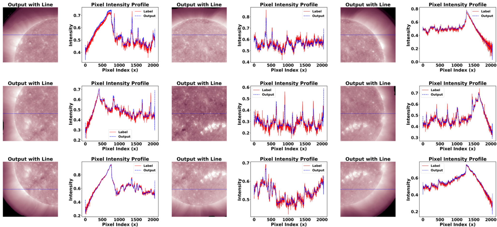
Figure 3. from Hao Li et al 2026 Astrophys. J. Suppl. 287 doi:10.3847/1538-4365/aea219 https://dx.doi.org/10.3847/1538-4365/aea219 © 2026. The Author(s). Published by the American Astronomical Society.
