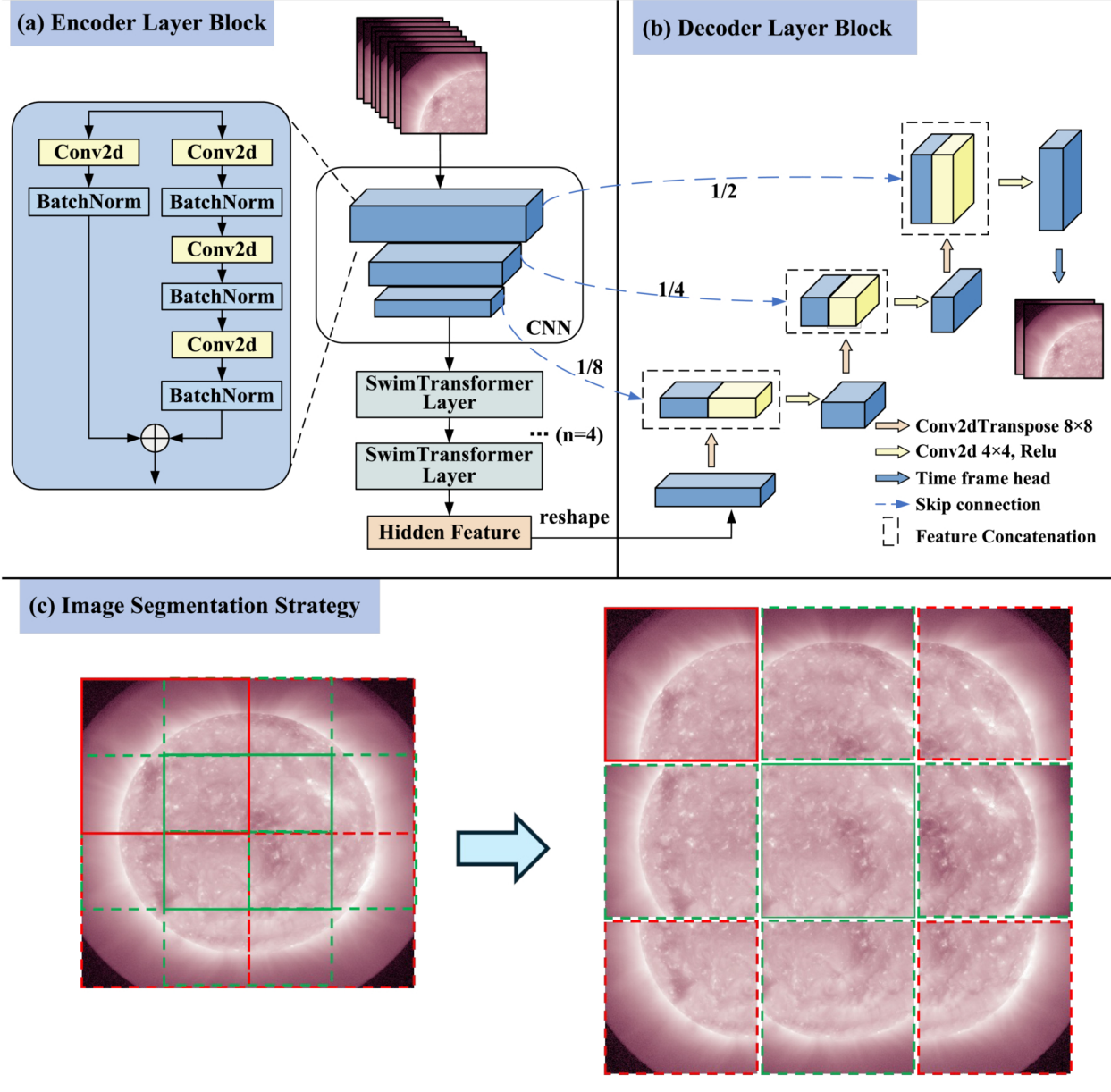
Figure 1. from Hao Li et al 2026 Astrophys. J. Suppl. 287 doi:10.3847/1538-4365/aea219 https://dx.doi.org/10.3847/1538-4365/aea219 © 2026. The Author(s). Published by the American Astronomical Society.
