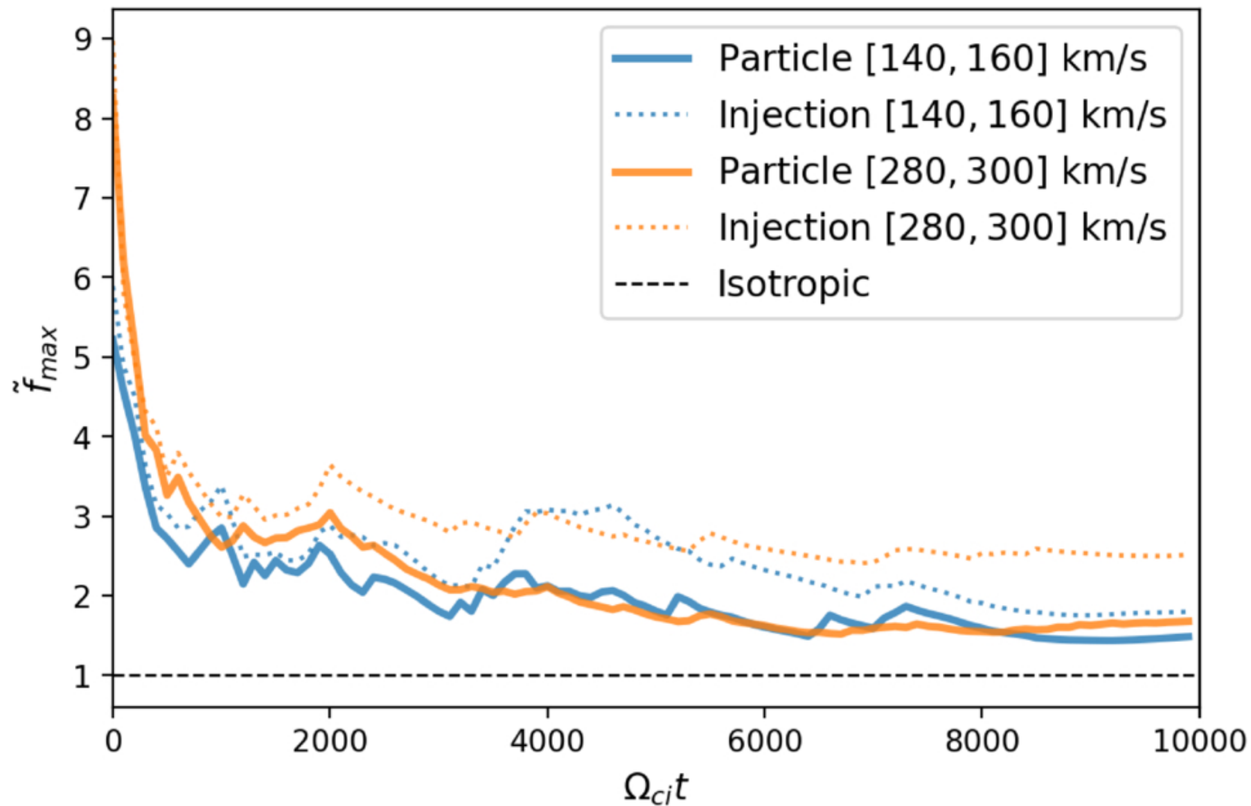
Figure 8. from Senbei Du et al 2026 Astrophys. J. Suppl. 286 doi:10.3847/1538-4365/aea206 https://dx.doi.org/10.3847/1538-4365/aea206 © 2026. The Author(s). Published by the American Astronomical Society.
