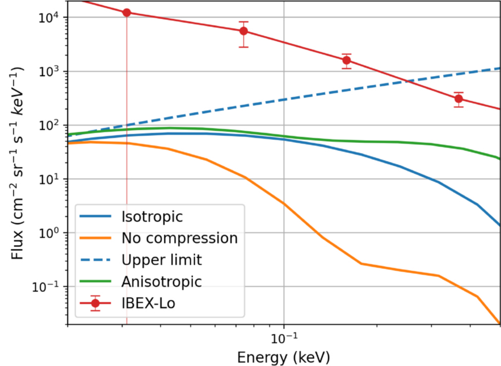
Figure 6. from Senbei Du et al 2026 Astrophys. J. Suppl. 286 doi:10.3847/1538-4365/aea206 https://dx.doi.org/10.3847/1538-4365/aea206 © 2026. The Author(s). Published by the American Astronomical Society.
