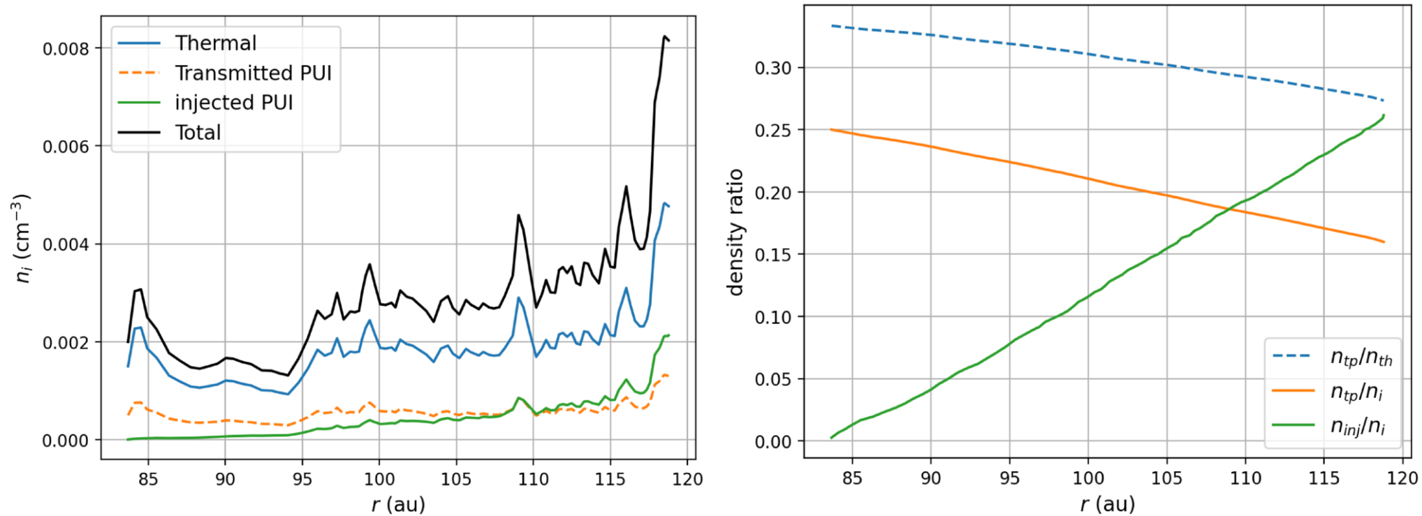
Figure 2. from Senbei Du et al 2026 Astrophys. J. Suppl. 286 doi:10.3847/1538-4365/aea206 https://dx.doi.org/10.3847/1538-4365/aea206 © 2026. The Author(s). Published by the American Astronomical Society.
