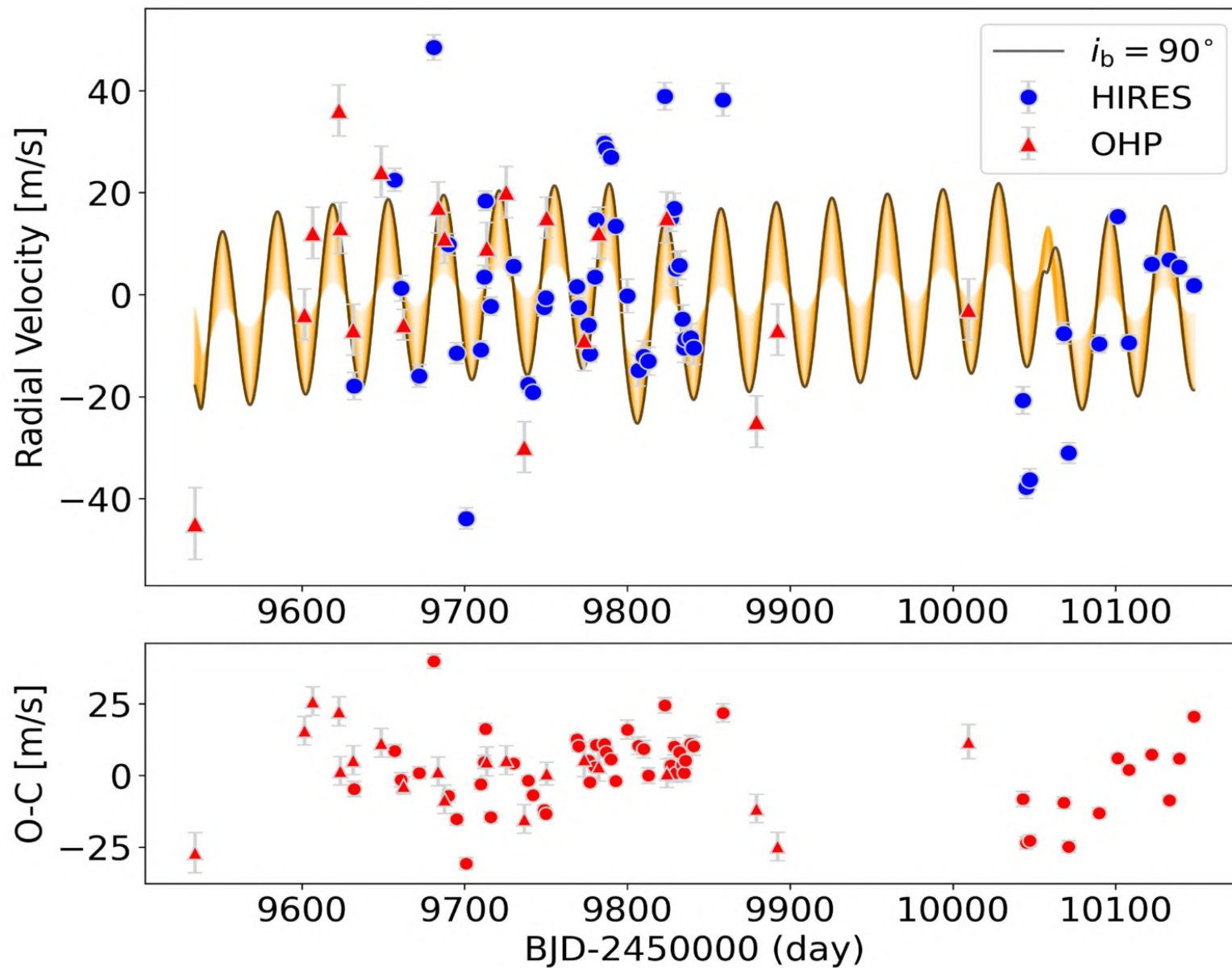
Figure 6. from Xiumin Huang and Jianghui Ji 2026 Astrophys. J. Suppl. 286 doi:10.3847/1538-4365/aea08b https://dx.doi.org/10.3847/1538-4365/aea08b © 2026. The Author(s). Published by the American Astronomical Society.
