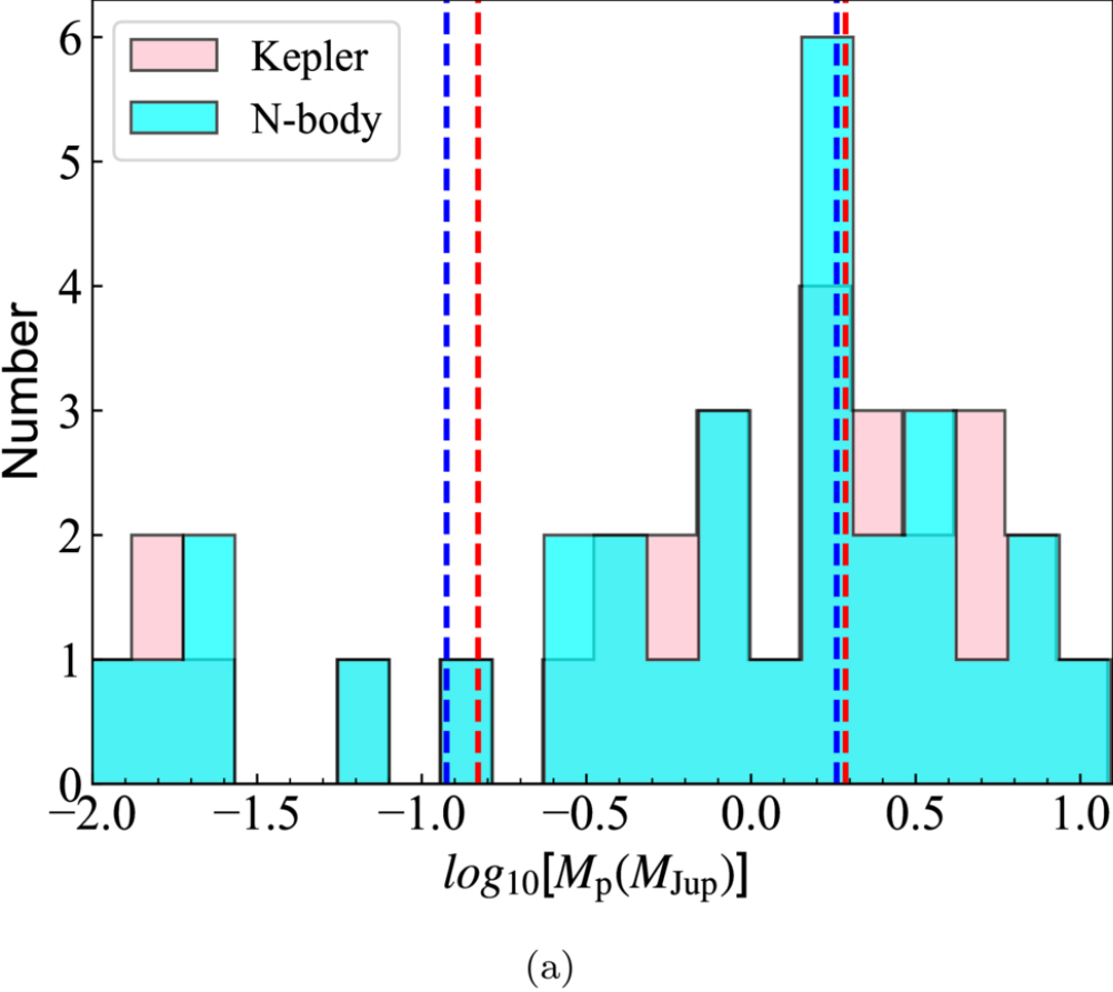
Figure 3. from Xiumin Huang and Jianghui Ji 2026 Astrophys. J. Suppl. 286 doi:10.3847/1538-4365/aea08b https://dx.doi.org/10.3847/1538-4365/aea08b © 2026. The Author(s). Published by the American Astronomical Society.
