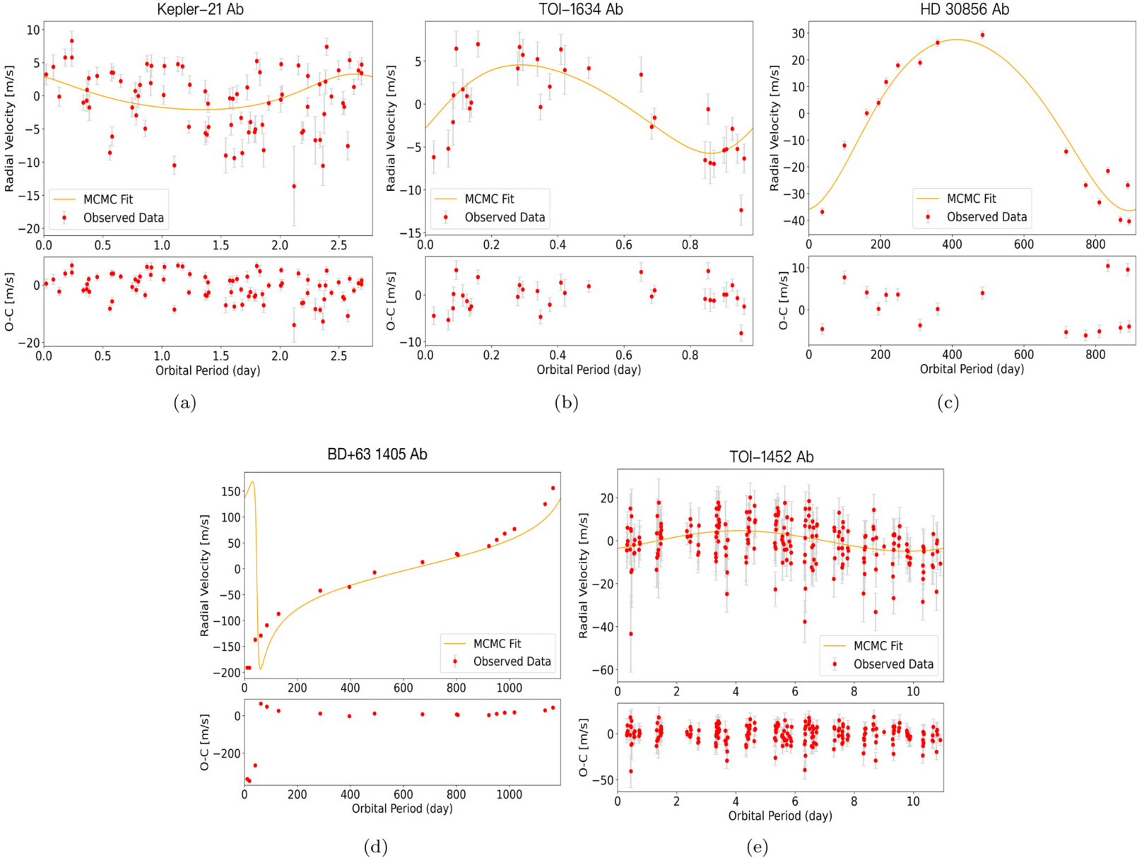
Figure B3. from Xiumin Huang and Jianghui Ji 2026 Astrophys. J. Suppl. 286 doi:10.3847/1538-4365/aea08b https://dx.doi.org/10.3847/1538-4365/aea08b © 2026. The Author(s). Published by the American Astronomical Society.
