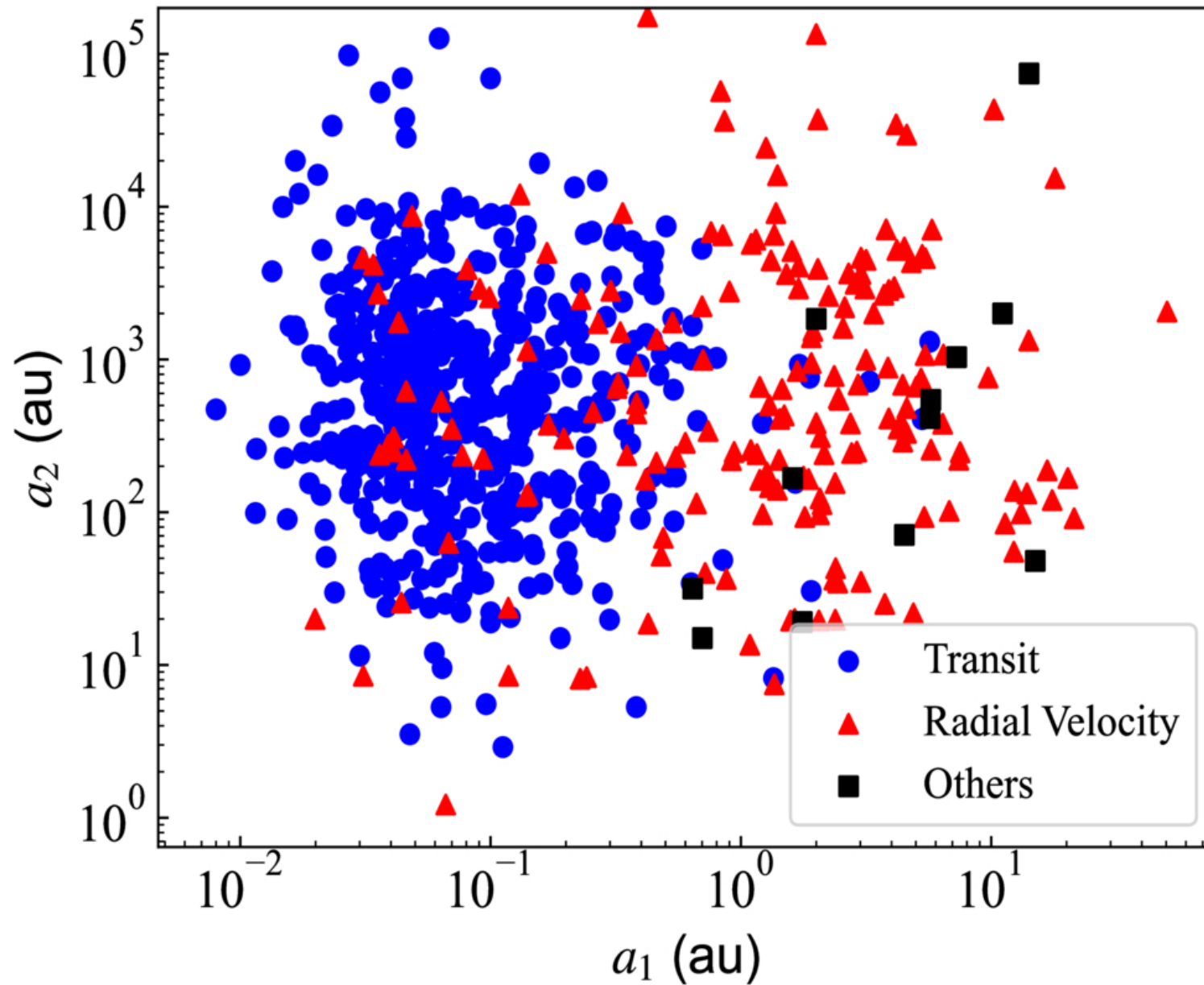
Figure 1. from Xiumin Huang and Jianghui Ji 2026 Astrophys. J. Suppl. 286 doi:10.3847/1538-4365/aea08b https://dx.doi.org/10.3847/1538-4365/aea08b © 2026. The Author(s). Published by the American Astronomical Society.
