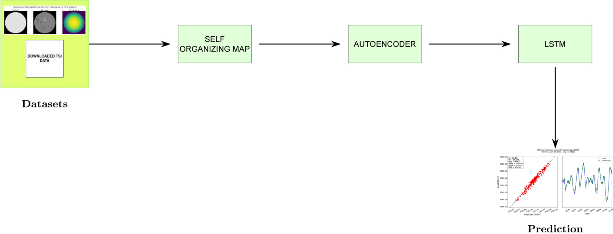
Figure 6. from Idowu Raji et al 2026 Astrophys. J. Suppl. 286 doi:10.3847/1538-4365/aea07a https://dx.doi.org/10.3847/1538-4365/aea07a © 2026. The Author(s). Published by the American Astronomical Society.
