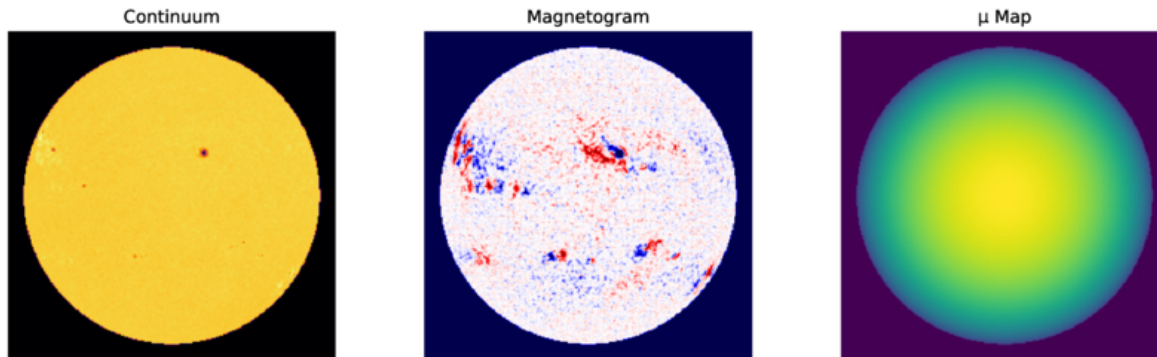
Visualization of SDO Image Channels: Continuum, Magnetogram, and \mu Map
