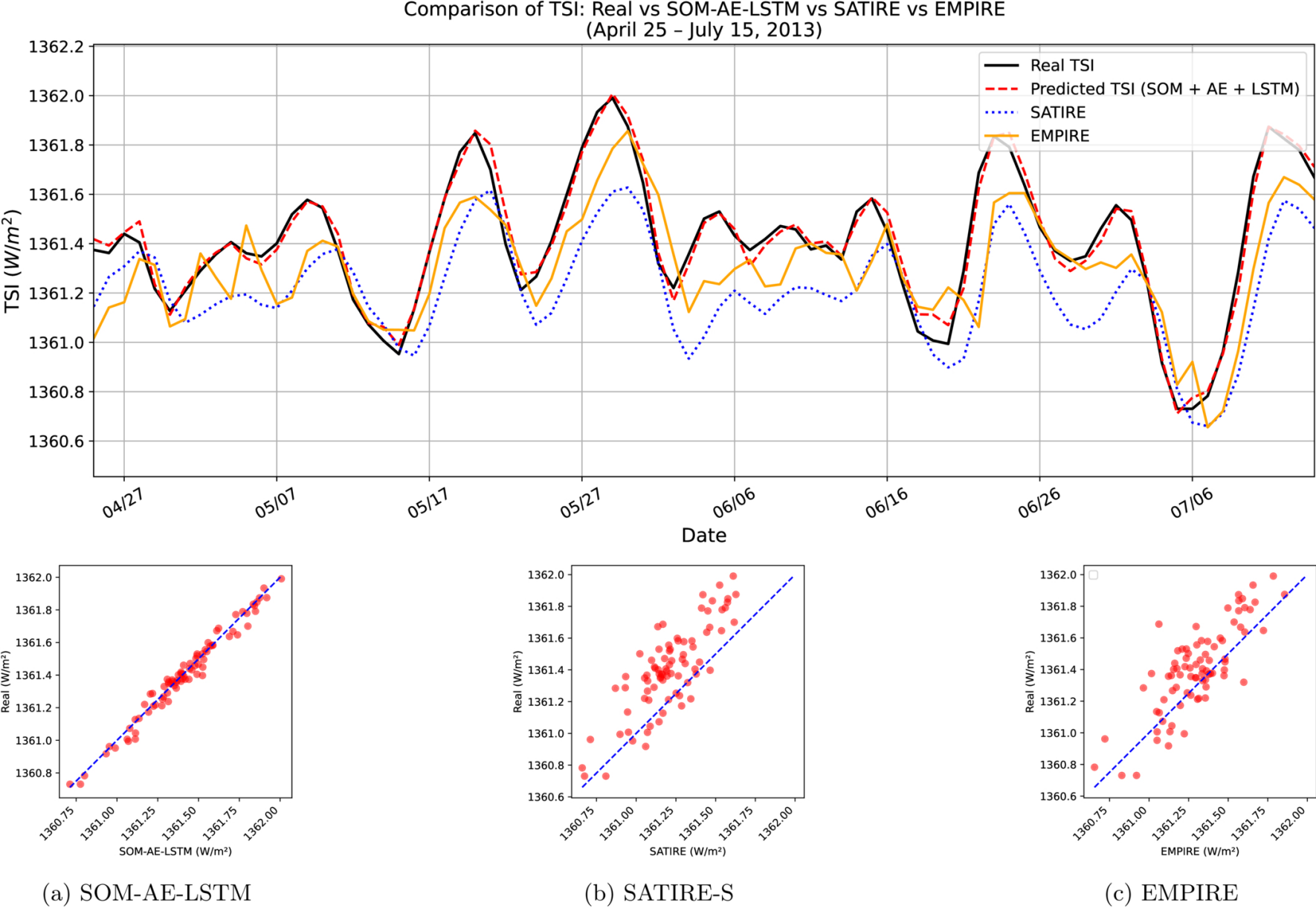
Figure 10. from Idowu Raji et al 2026 Astrophys. J. Suppl. 286 doi:10.3847/1538-4365/aea07a https://dx.doi.org/10.3847/1538-4365/aea07a © 2026. The Author(s). Published by the American Astronomical Society.
