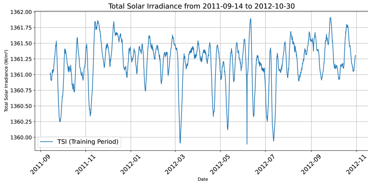
Figure 1. from Idowu Raji et al 2026 Astrophys. J. Suppl. 286 doi:10.3847/1538-4365/aea07a https://dx.doi.org/10.3847/1538-4365/aea07a © 2026. The Author(s). Published by the American Astronomical Society.
