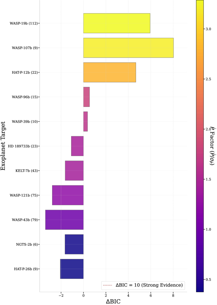
Figure 7. from Yunke Wu et al 2026 Astrophys. J. Suppl. 287 doi:10.3847/1538-4365/aea075 https://dx.doi.org/10.3847/1538-4365/aea075 © 2026. The Author(s). Published by the American Astronomical Society.
