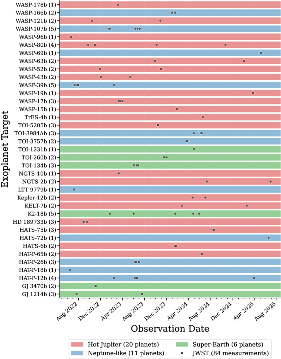
Figure 3. from Yunke Wu et al 2026 Astrophys. J. Suppl. 287 doi:10.3847/1538-4365/aea075 https://dx.doi.org/10.3847/1538-4365/aea075 © 2026. The Author(s). Published by the American Astronomical Society.
