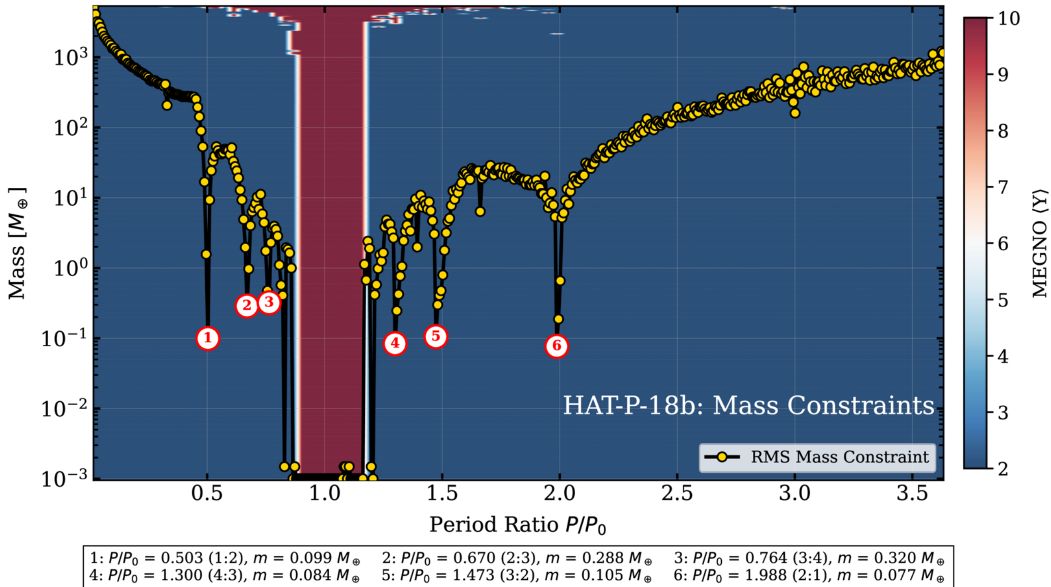
Figure 20. from Yunke Wu et al 2026 Astrophys. J. Suppl. 287 doi:10.3847/1538-4365/aea075 https://dx.doi.org/10.3847/1538-4365/aea075 © 2026. The Author(s). Published by the American Astronomical Society.
