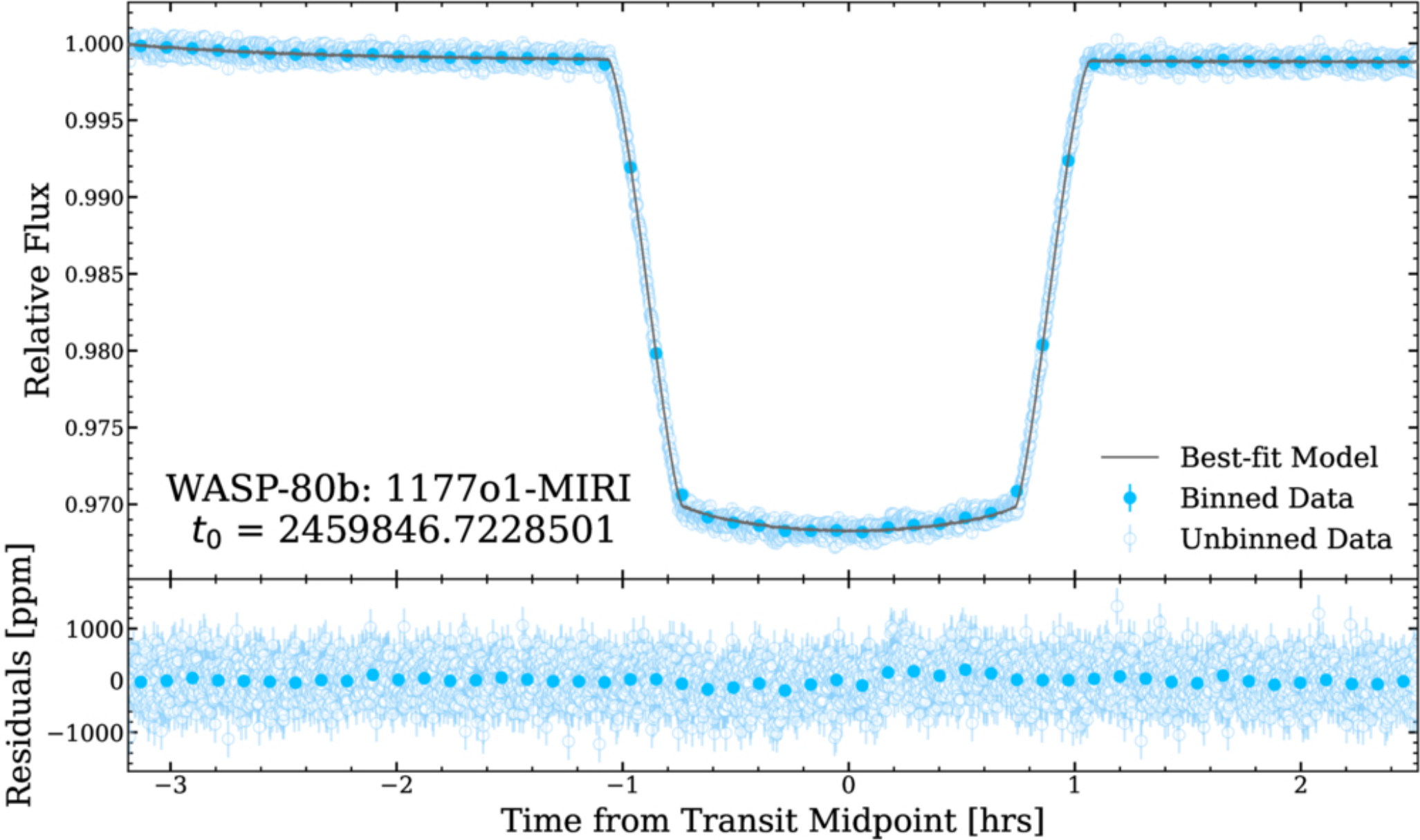
Figure 2. from Yunke Wu et al 2026 Astrophys. J. Suppl. 287 doi:10.3847/1538-4365/aea075 https://dx.doi.org/10.3847/1538-4365/aea075 © 2026. The Author(s). Published by the American Astronomical Society.
