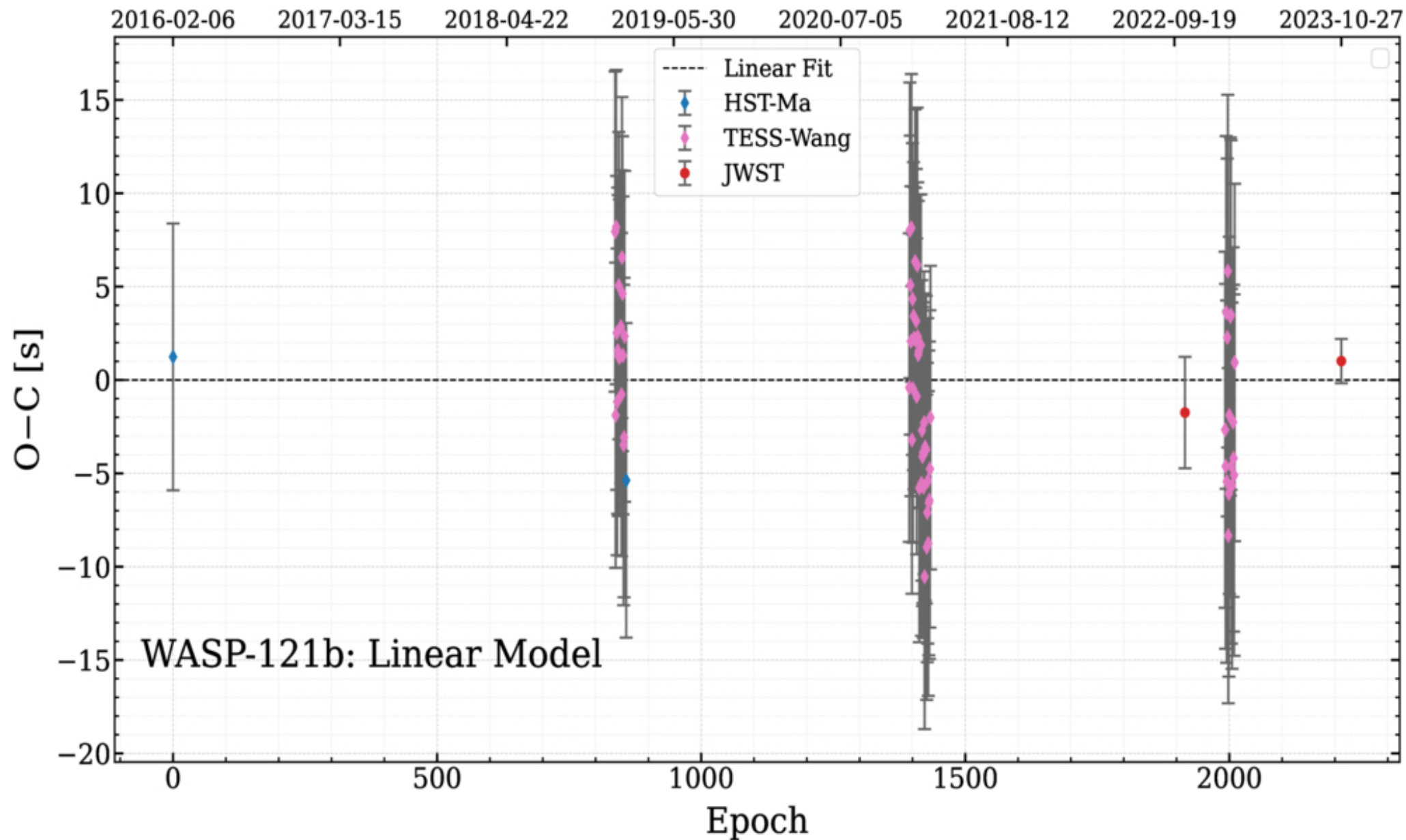
Figure 19. from Yunke Wu et al 2026 Astrophys. J. Suppl. 287 doi:10.3847/1538-4365/aea075 https://dx.doi.org/10.3847/1538-4365/aea075 © 2026. The Author(s). Published by the American Astronomical Society.
